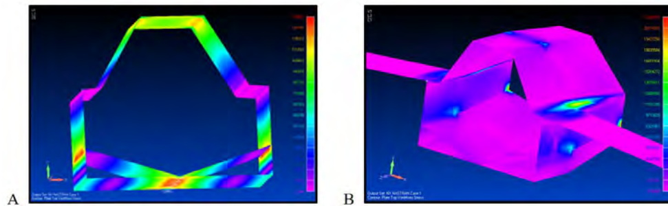
Figure 11 - FE models – (A) First model, thin extruded 2D shape, (B) Final model, 3D shape
