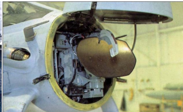
Figure 12. AN/APQ-126 TF/TA radar
