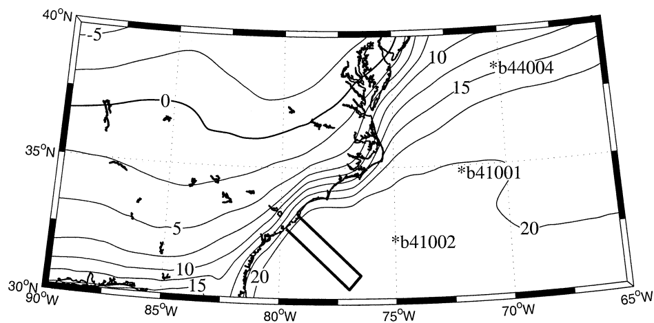
FIG. 4. Location of GALE IOP2 (box) and National Buoy Data Center (asterisks) data. The background field is the monthly mean surface temperature field ( ^{\circ}\text{C} ) for Jan from the NCEP–NCAR reanalysis.
