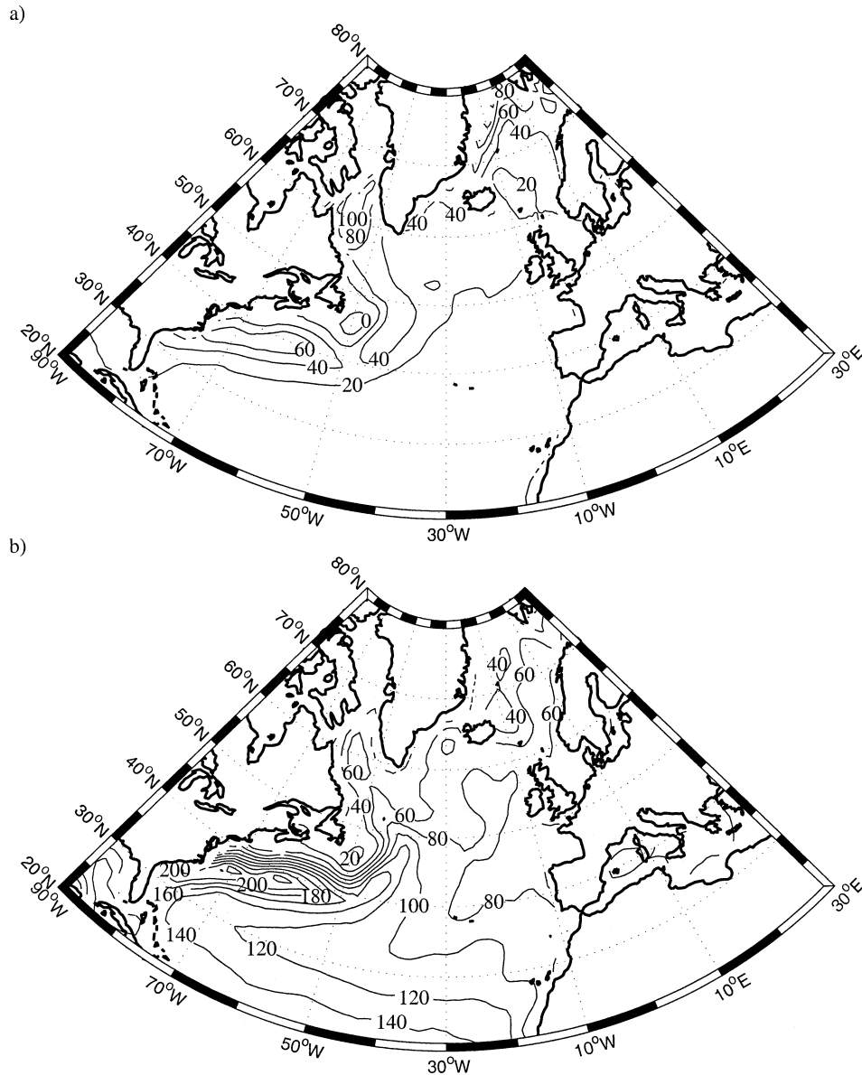
FIG. 1. Annual mean (a) sensible and (b) latent heat fluxes ( \text{W m}^{-2} ) from the NCEP-NCAR reanalysis over the North Atlantic Ocean. Climatology based on years 1979–93.
