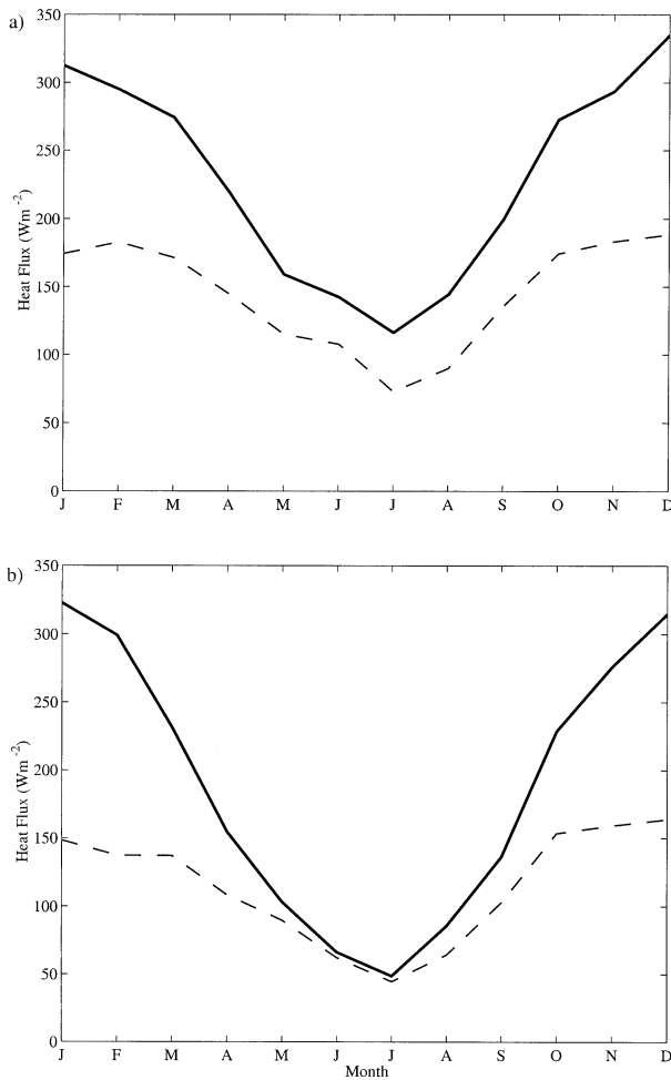
FIG. 3. Annual cycle of monthly mean latent heat flux (solid line) and monthly mean std dev of the 6-hourly latent heat flux (dashed line) at (a) 37^{\circ}\text{N} , 70^{\circ}\text{W} and (b) 35^{\circ}\text{N} , 144^{\circ}\text{E} .
