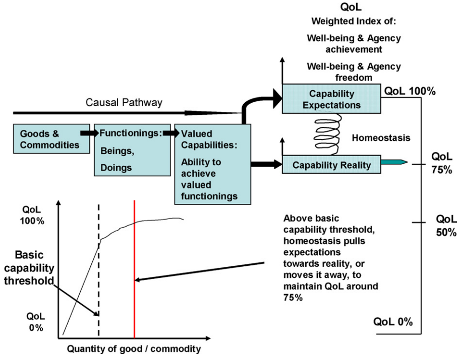
Fig. 4. Quality of life is maintained at around 75% when availability of goods and commodities raises capability reality above basic threshold.
