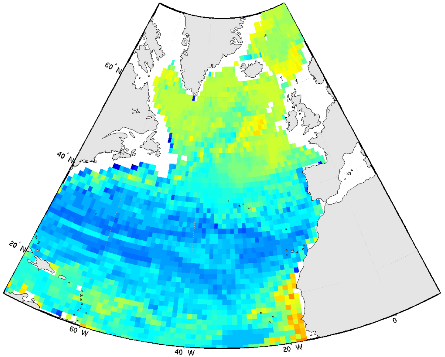
pCO 2 - march2006
