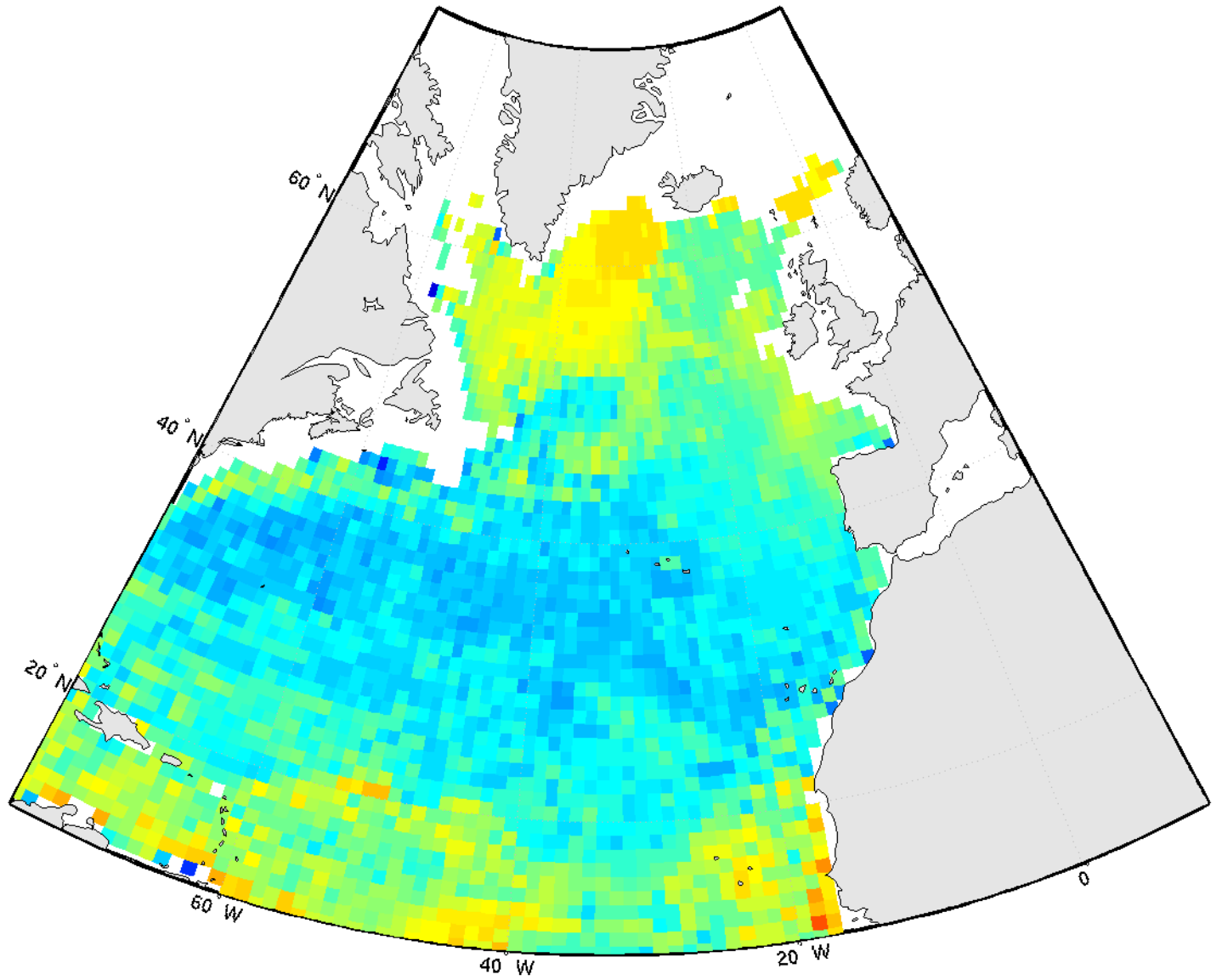
pCO 2 - february2005
