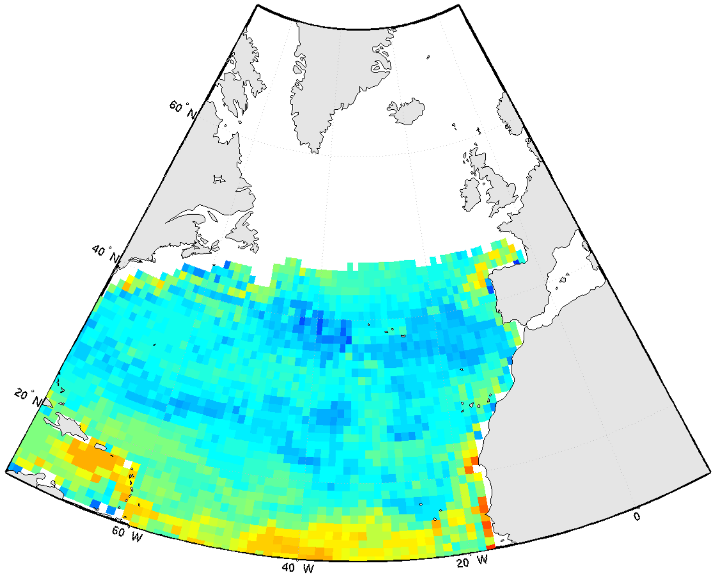
pCO 2 - december2006
