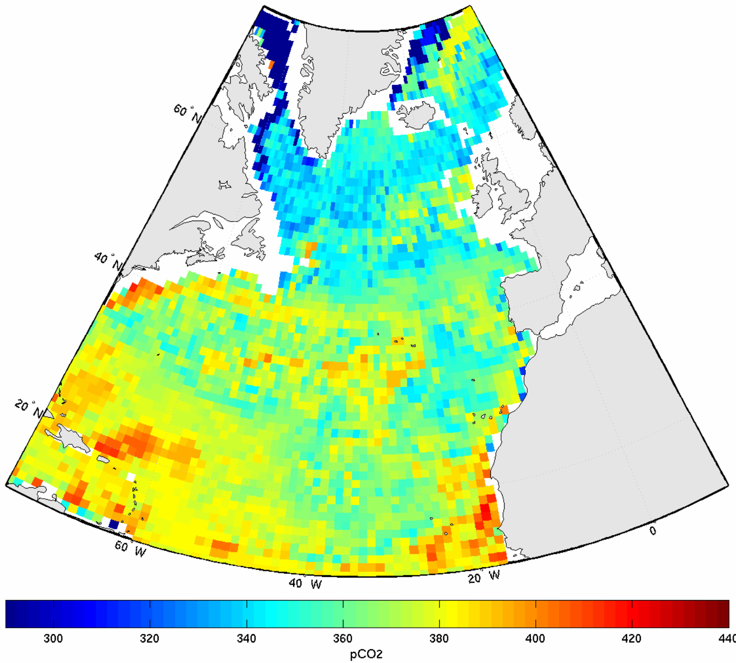
pCO 2 - september2005
