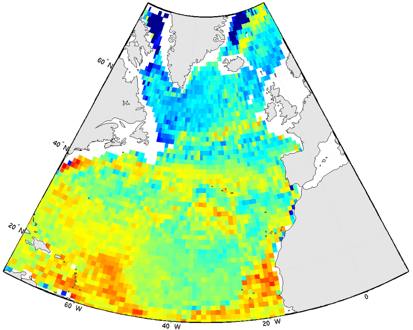
pCO 2 - september2004
