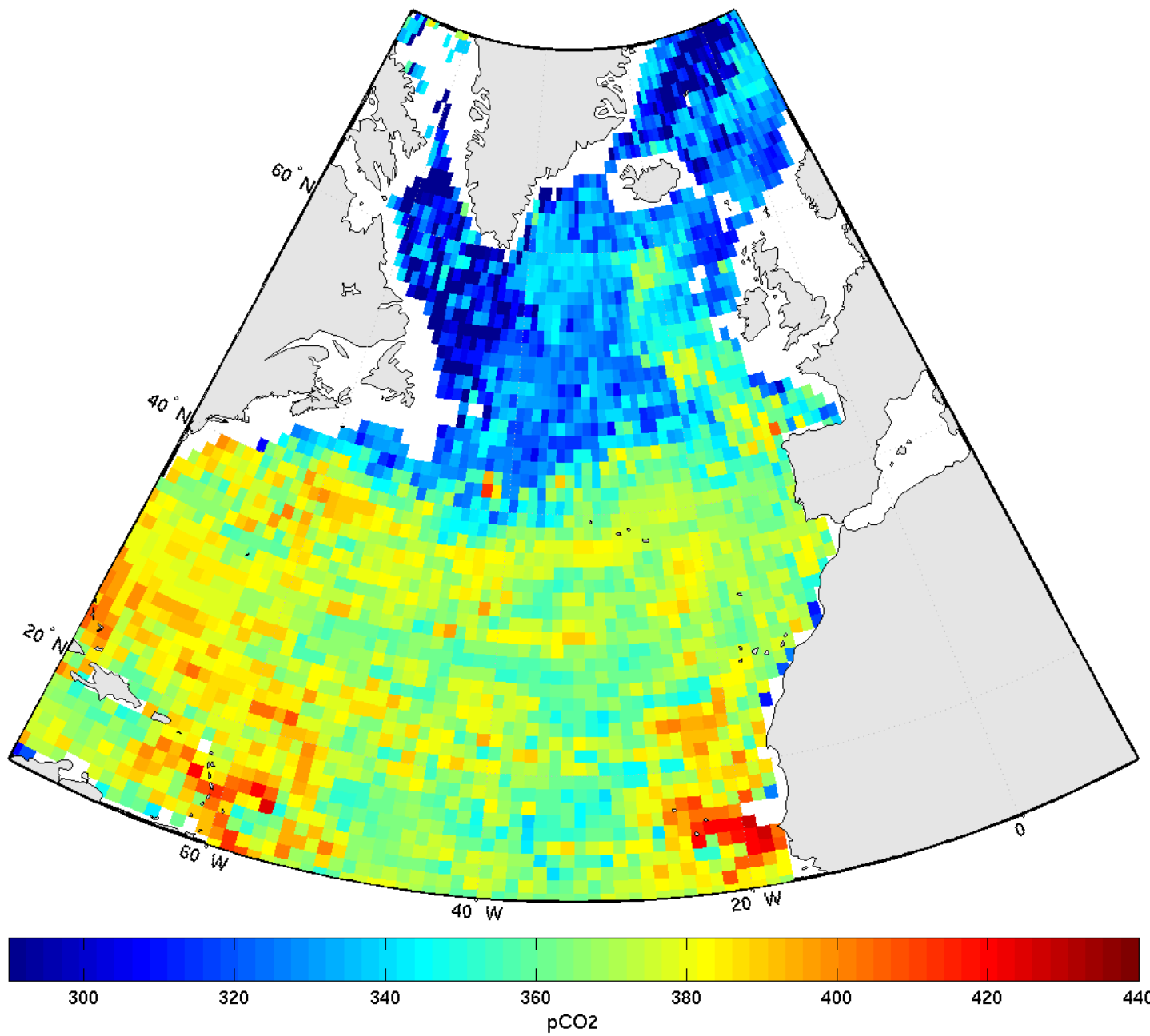
pCO 2 - june2004
