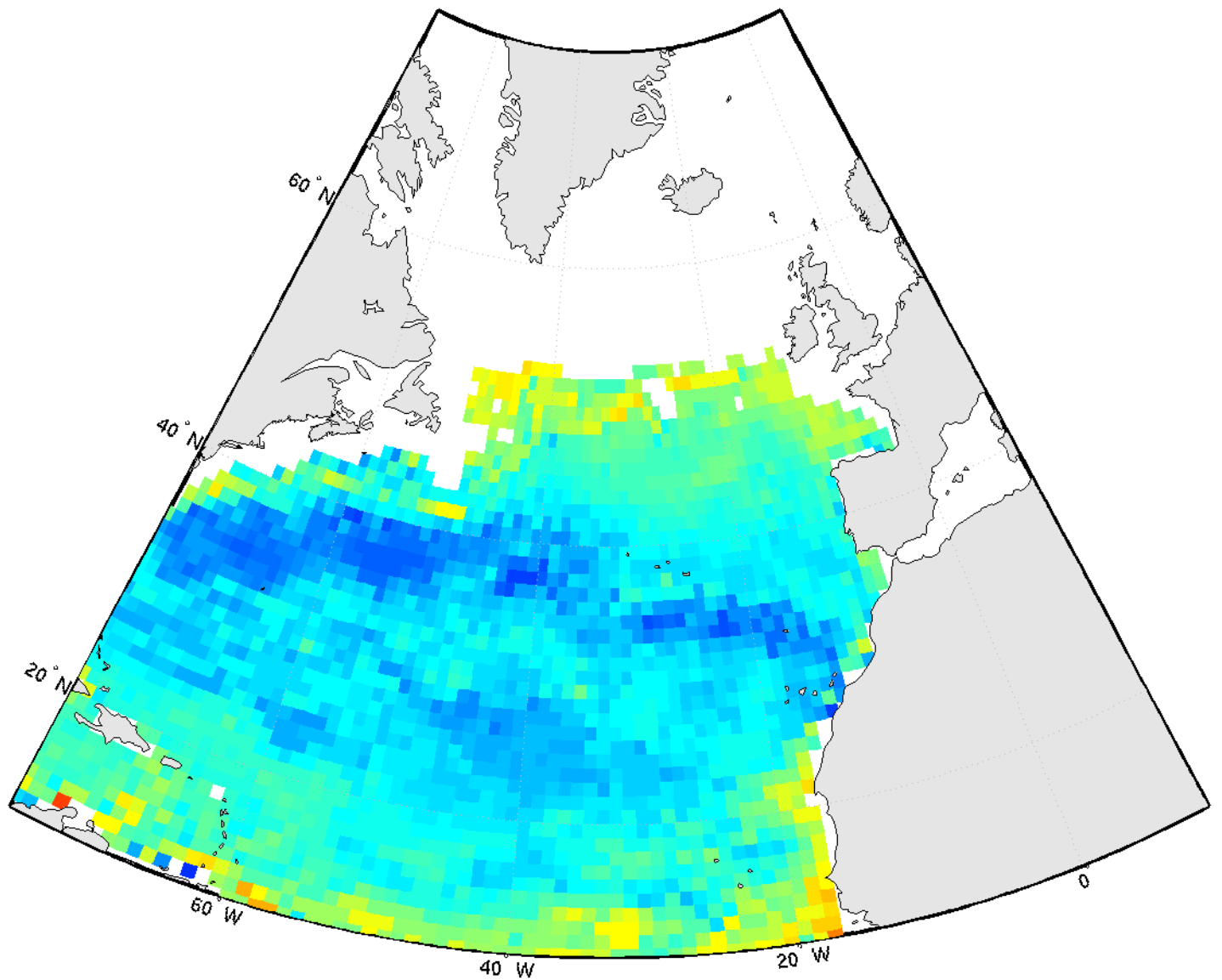
pCO 2 - january2006
