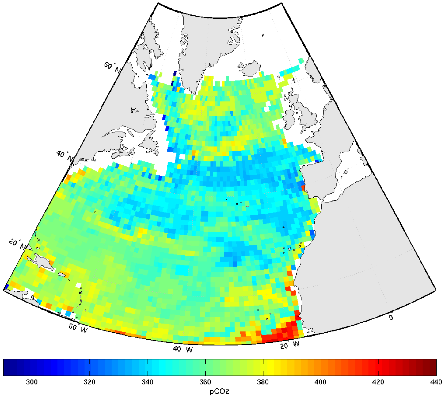
pCO 2 - october2005
