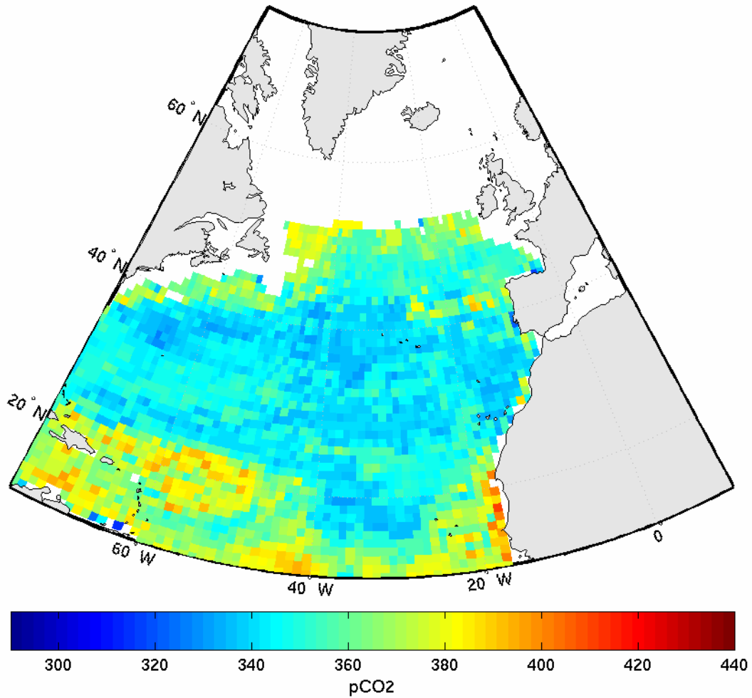
pCO 2 - january2004
