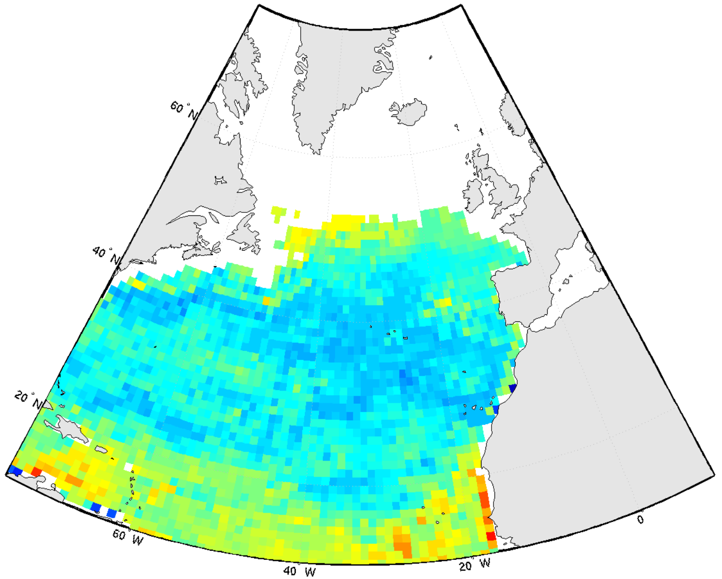
pCO 2 - january2005
