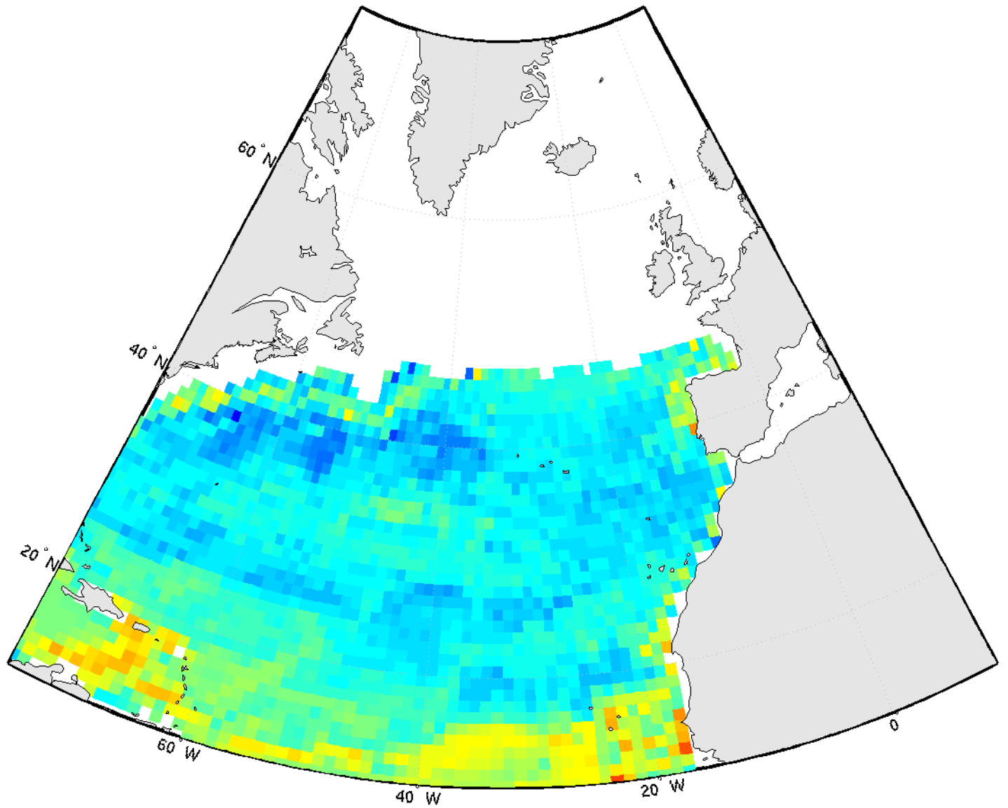
pCO 2 - december2005
