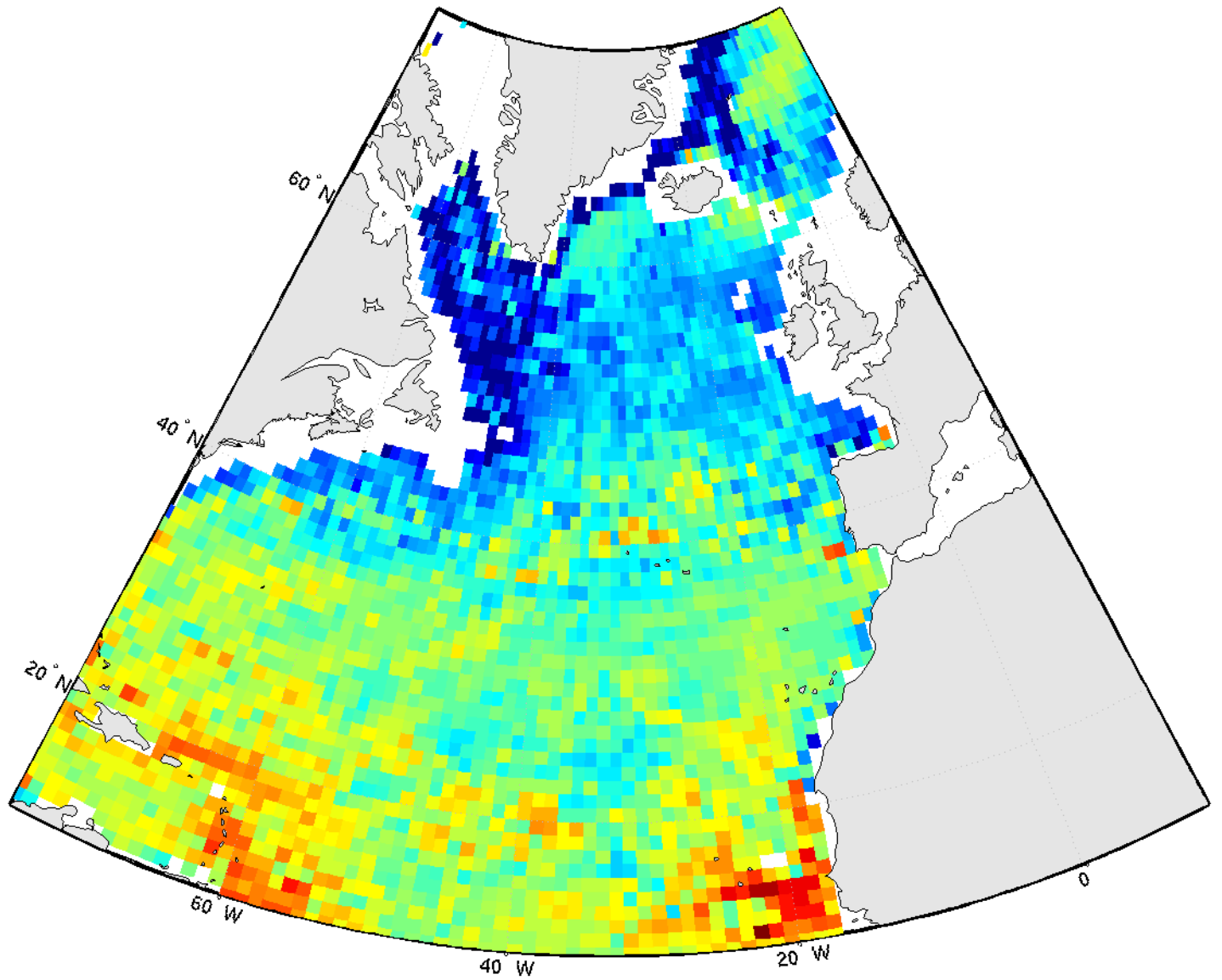
pCO 2 - may2005
