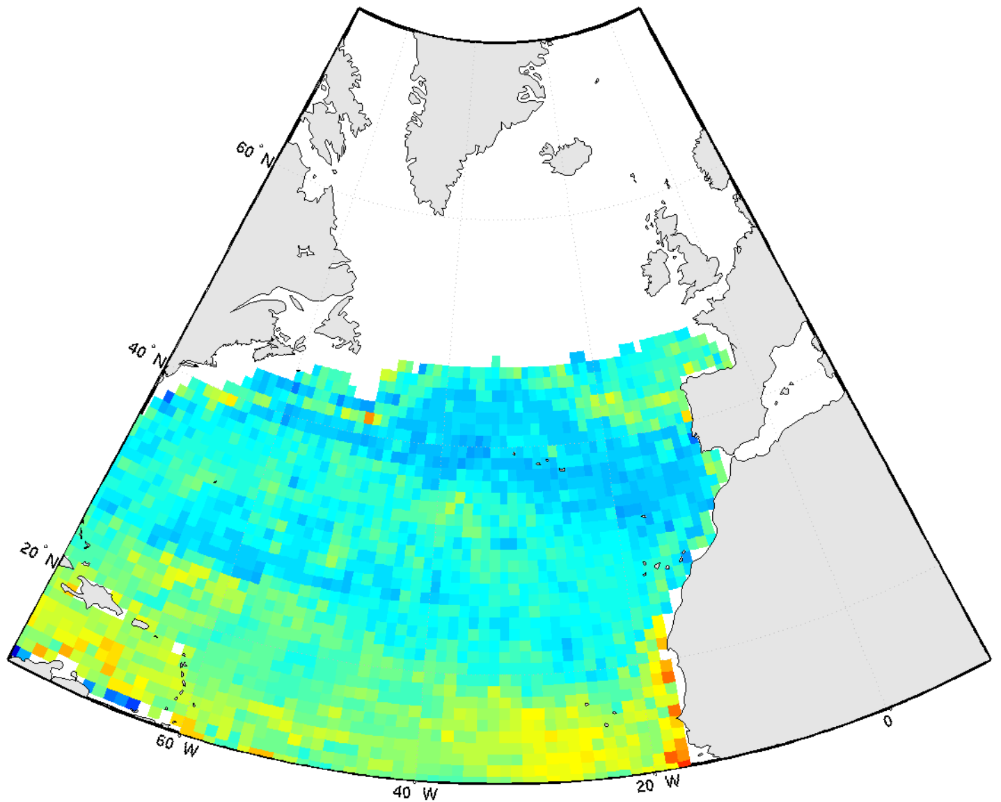
pCO 2 - december2004
