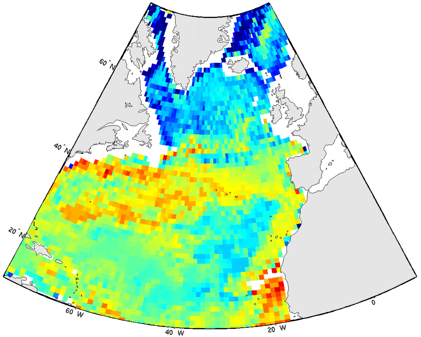
pCO 2 - july2006
