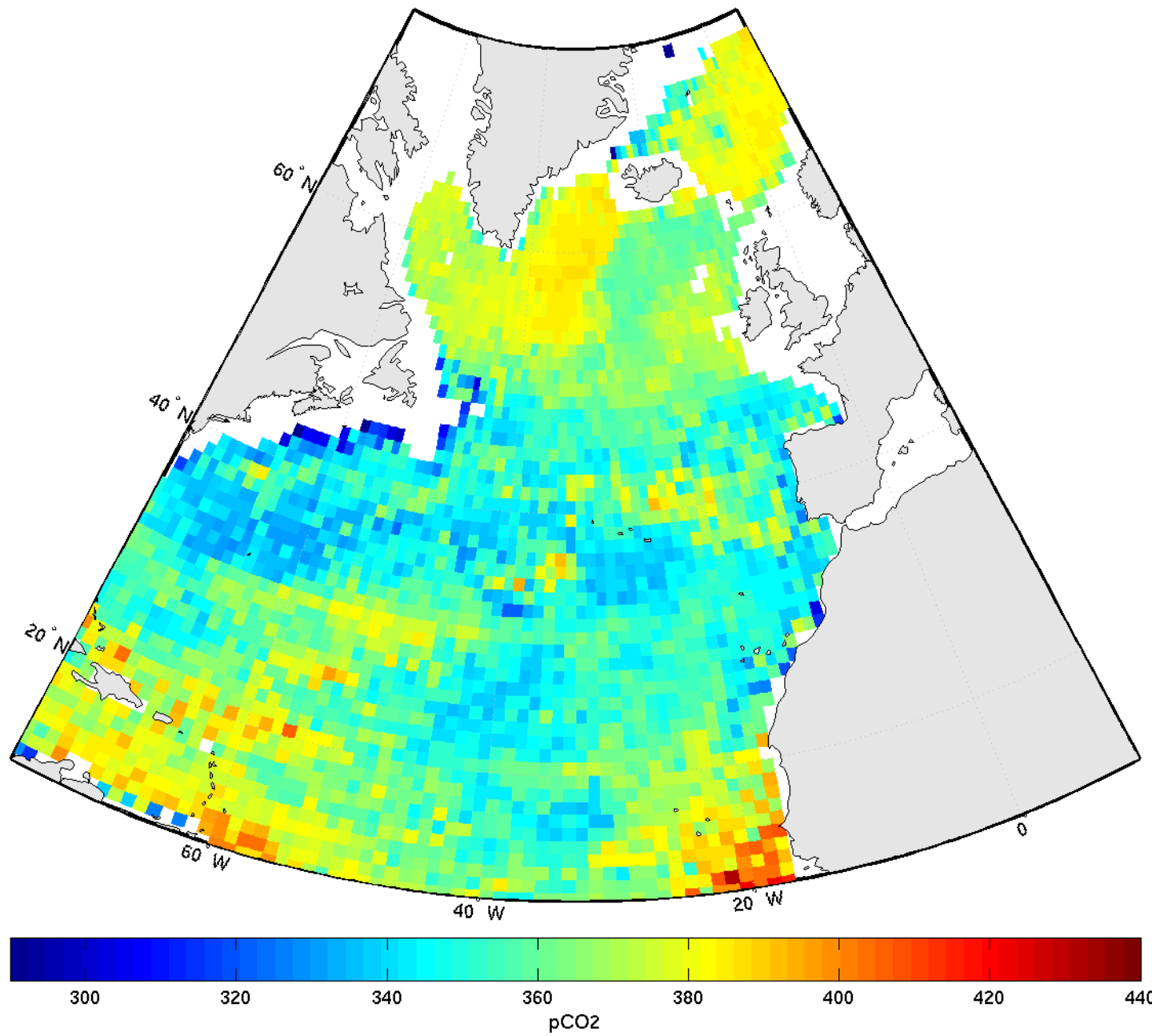
pCO 2 - march2004
