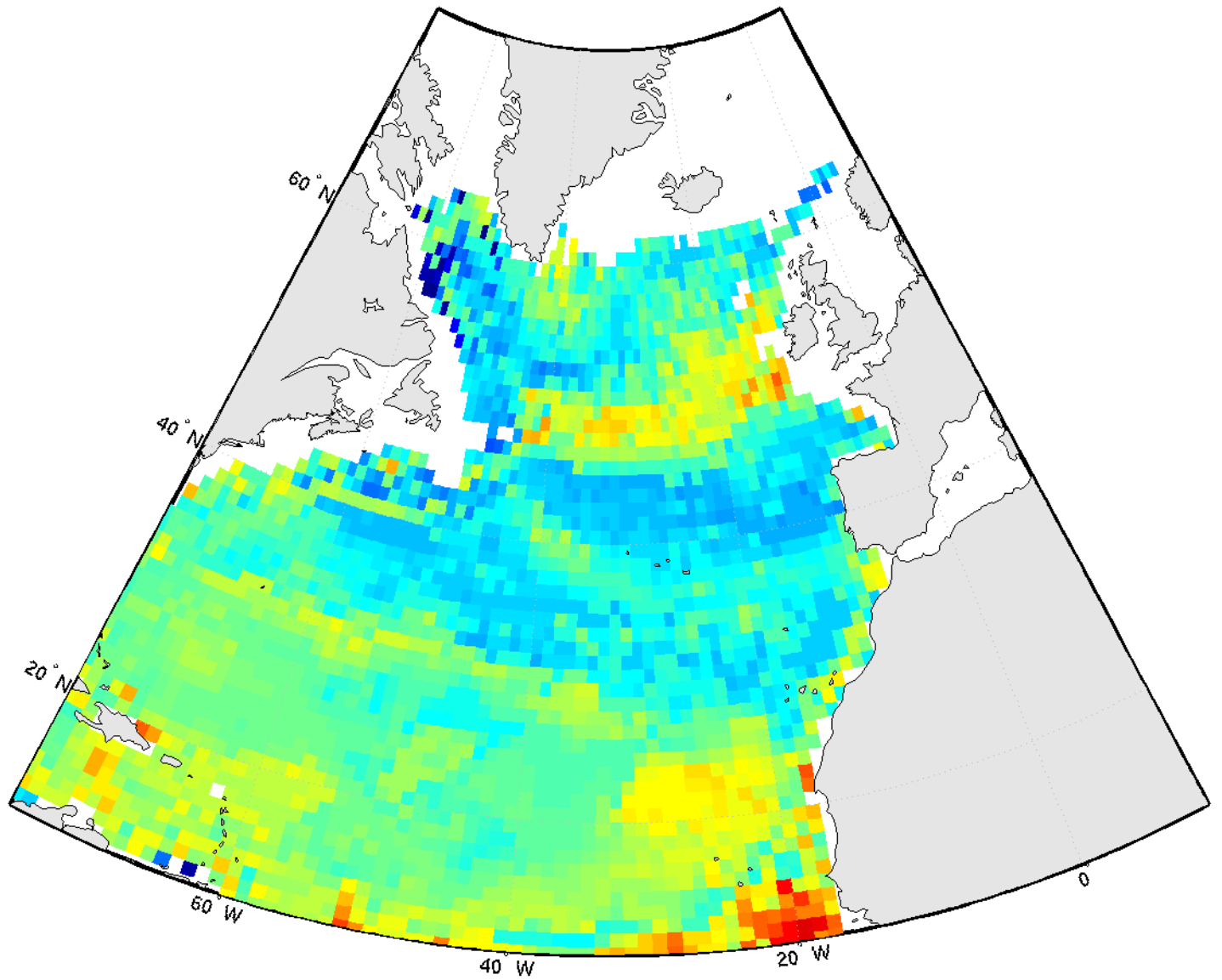
pCO 2 - october2006
