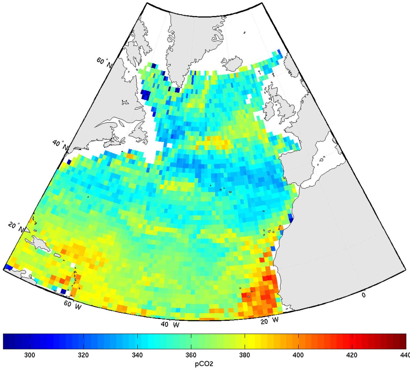
pCO 2 - october2004
