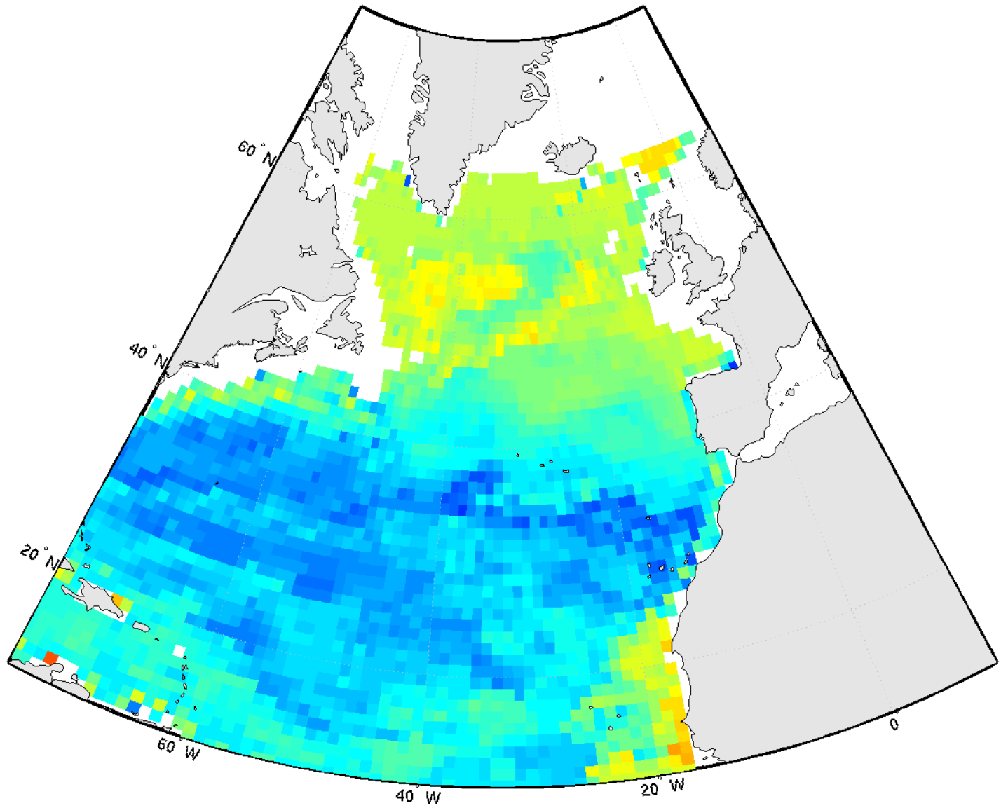
pCO 2 - february2006
