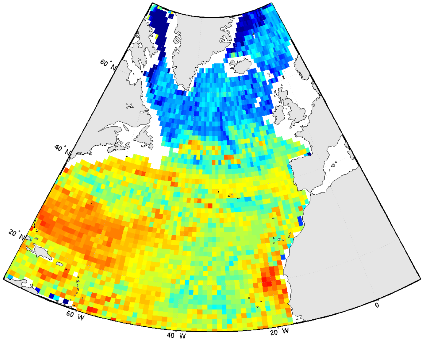
pCO 2 - august2004
