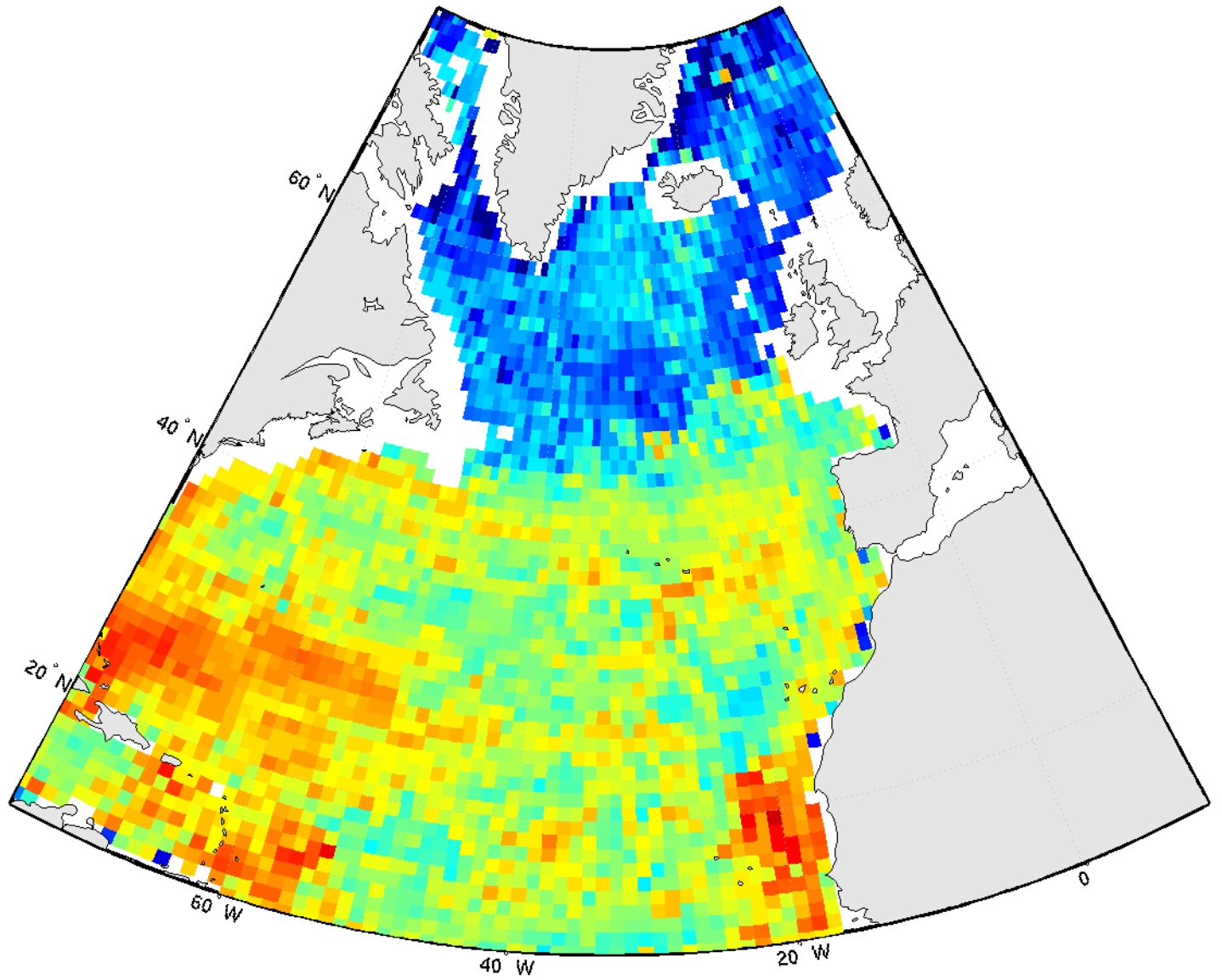
pCO 2 - july2004
