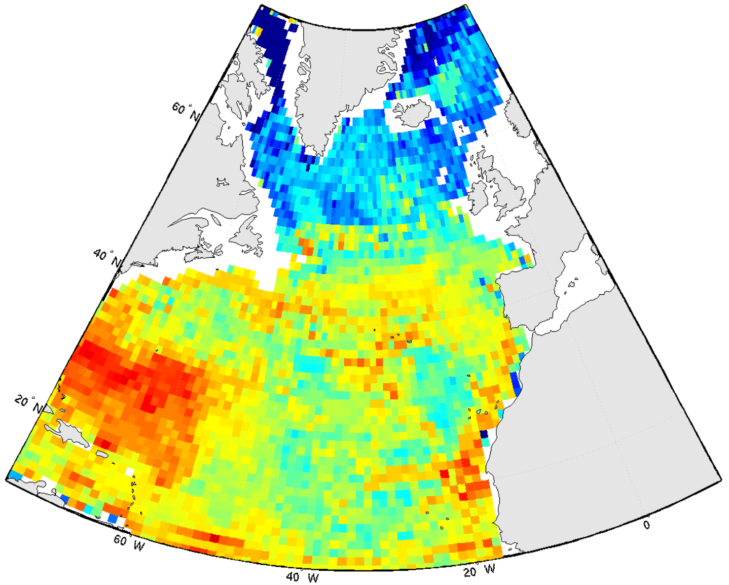
pCO 2 - august2005
