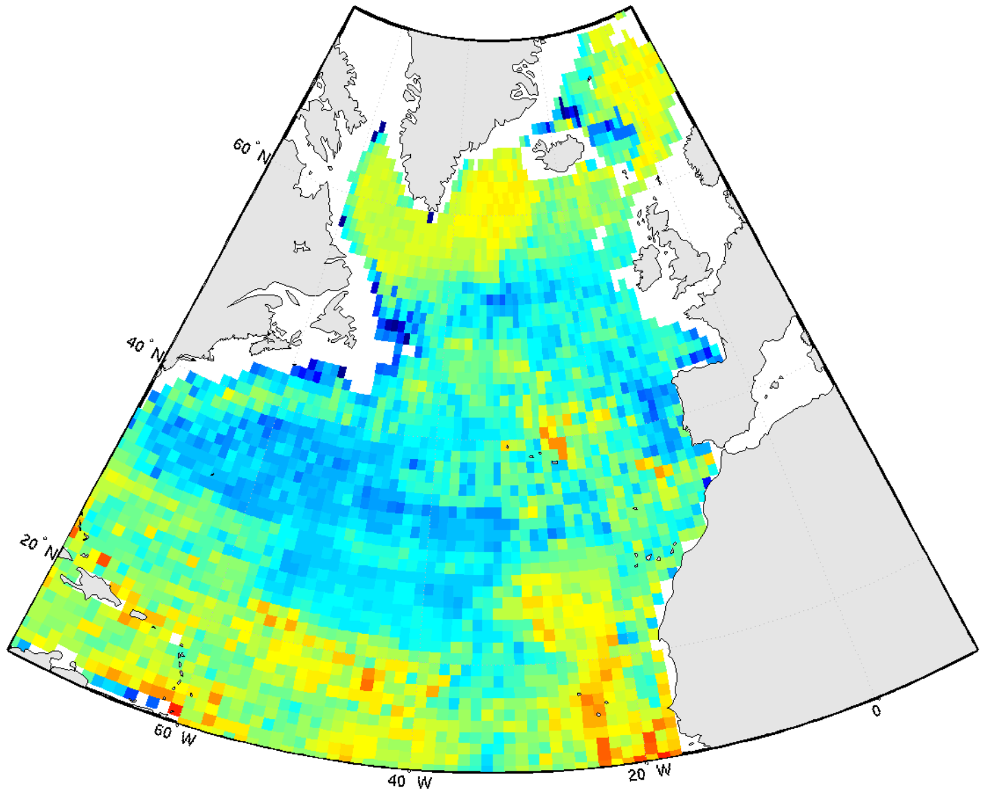
pCO 2 - march2005
