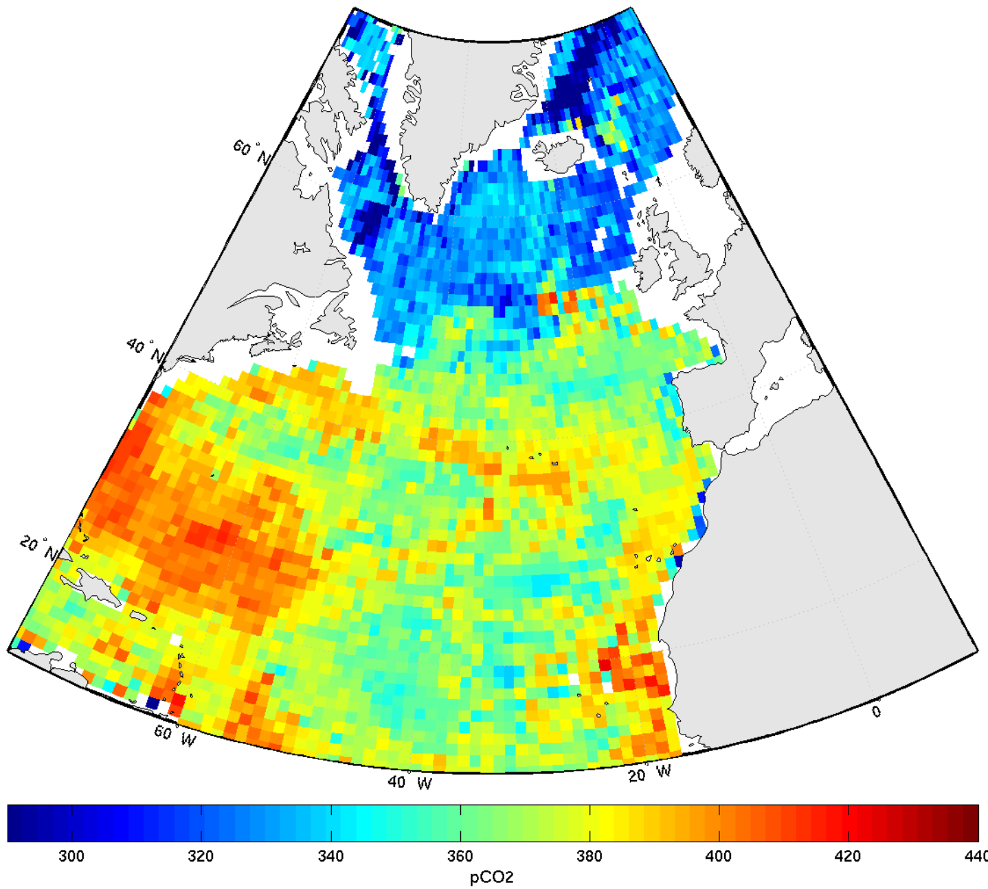
pCO 2 - july2005
