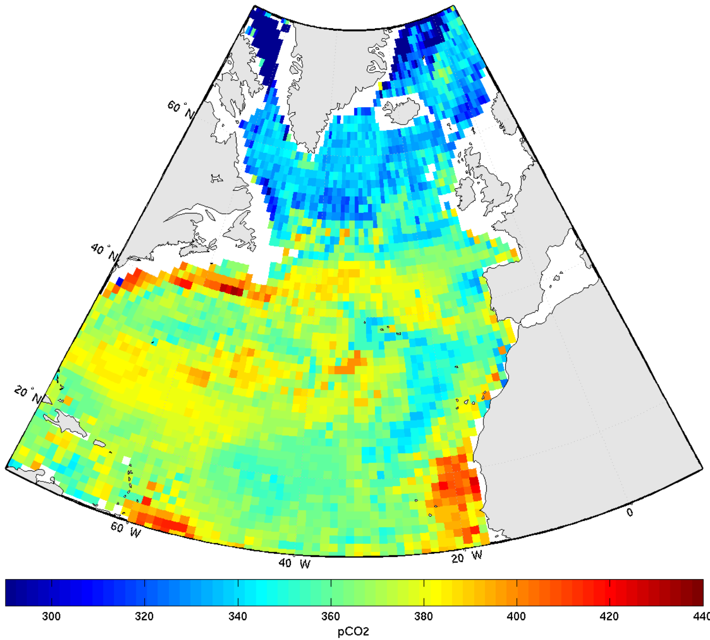
pCO 2 - august2006
