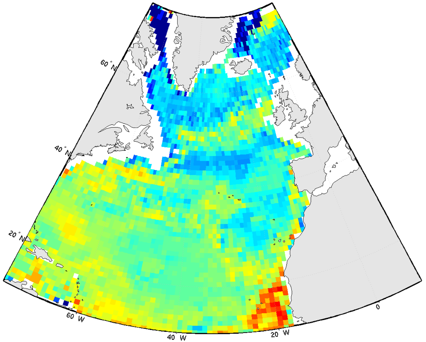
pCO 2 - september2006
