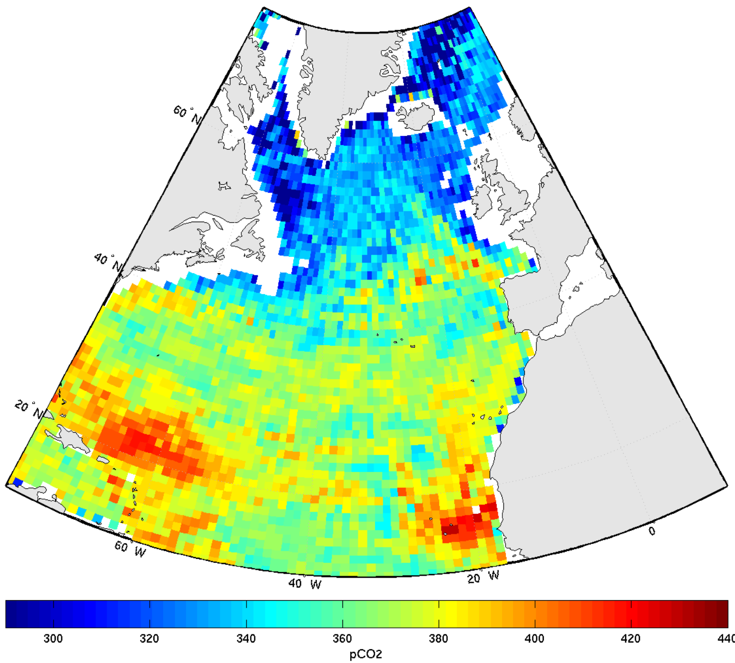
pCO 2 - june2005
