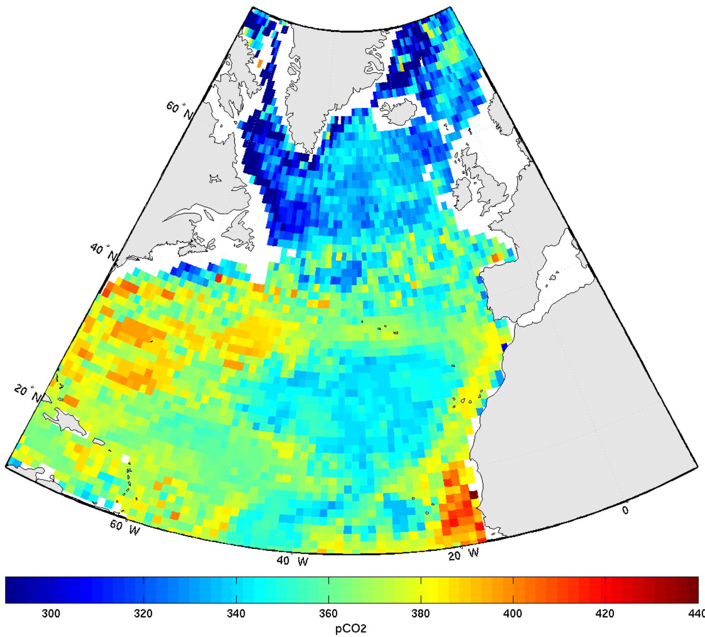
pCO 2 - june2006
