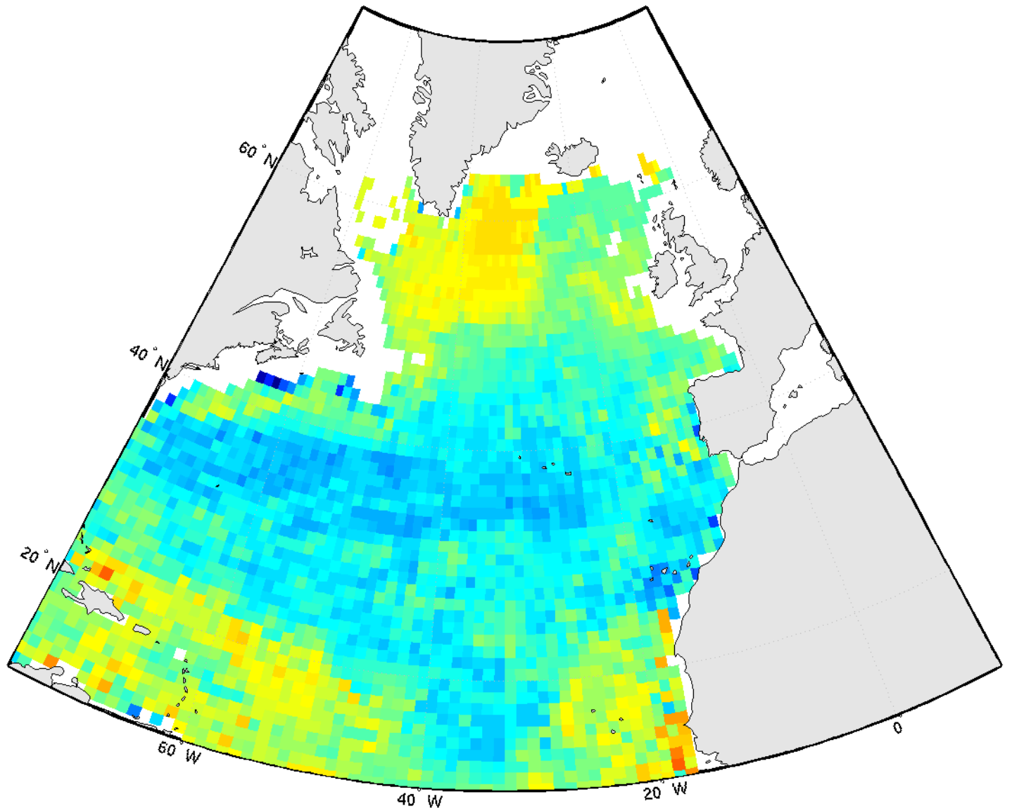
pCO 2 - february2004
