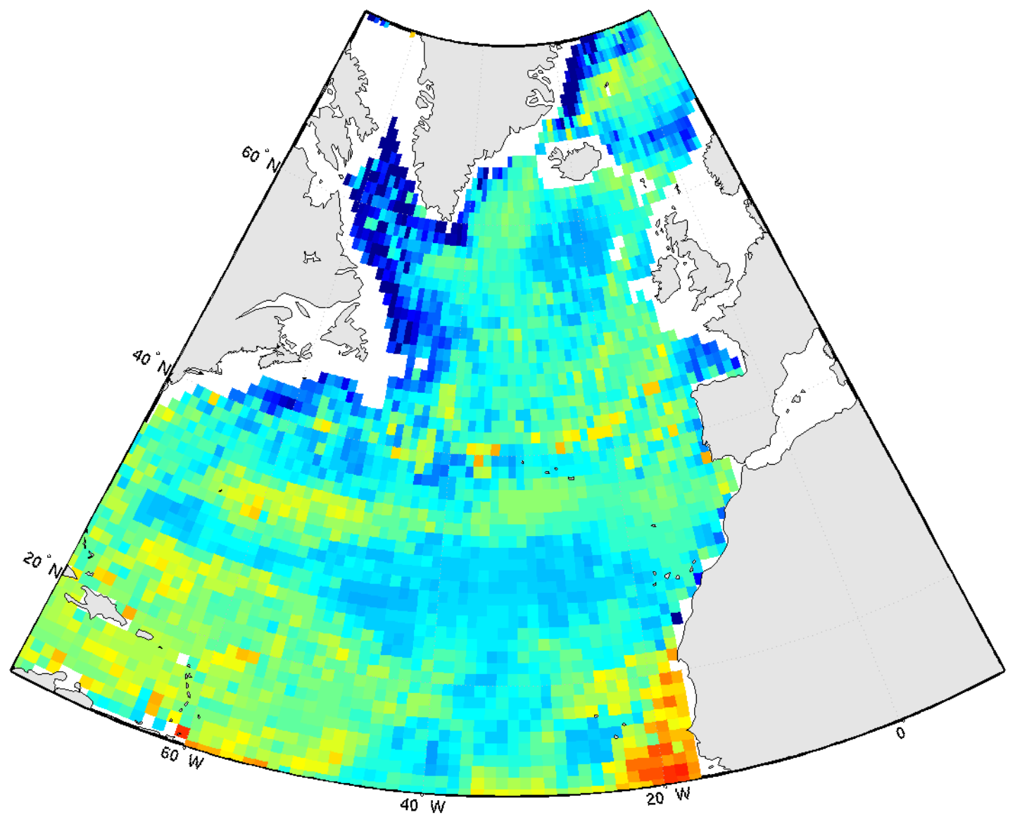
pCO 2 - may2006
