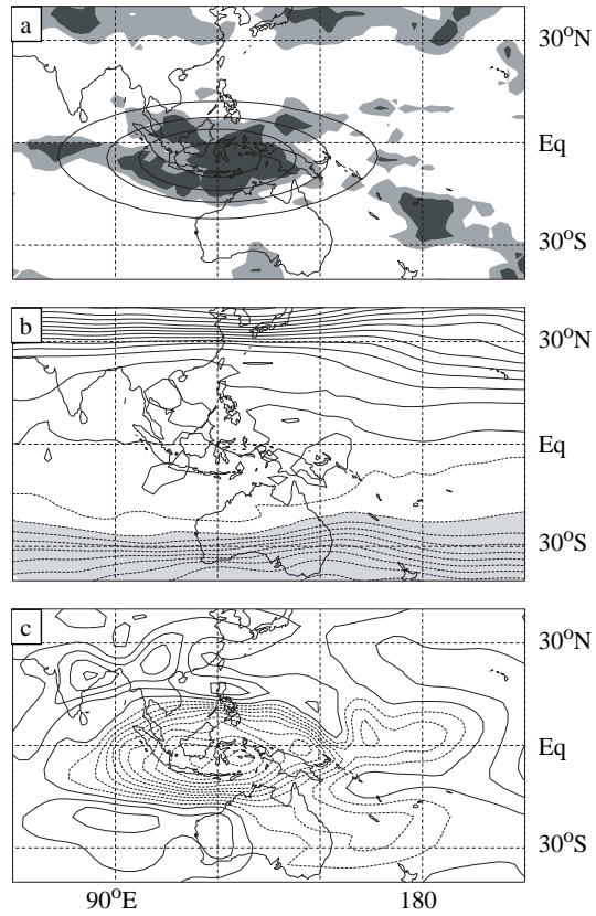
Figure 11. (a) Idealised heating shape, together with the OLR field of 26 March 1988, shaded (darkly) below 225 (175) \text{W m}^{-2} . (b) Total potential vorticity at 355K (shaded below -1 PVU; contour interval is 0.5 PVU) and (c) perturbation omega at 500 mb (contour interval is 0.5 \text{ mb hr}^{-1} ), both on day 3 of the integration. Positive (negative) contours are solid (dashed) and the zero contour is in bold.
