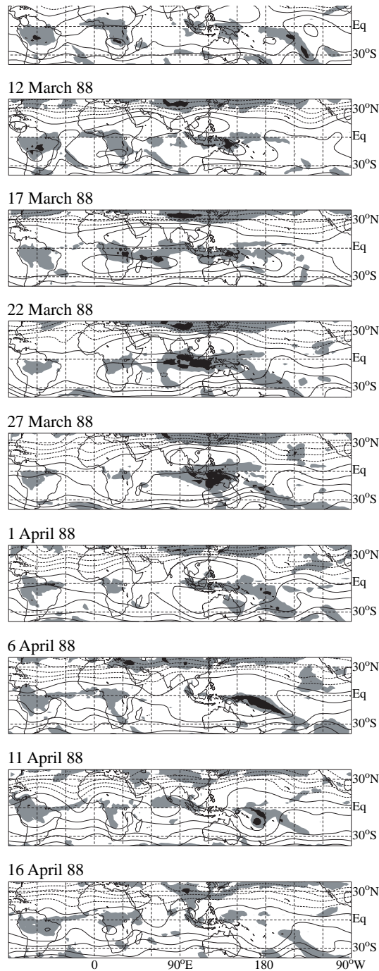
Figure 1. Pentad mean OLR and 355K streamfunction for the period 5 March - 18 April 1988. The date indicates the middle day of the pentad. OLR is shaded (darkly) below the 225 ( 175 ) \text{W m}^{-2} level. Streamfunction contours are every 2 \times 10^7 \text{ m}^2 \text{ s}^{-1} ; positive (negative) contours are solid (dashed) and the zero contour is in bold.
