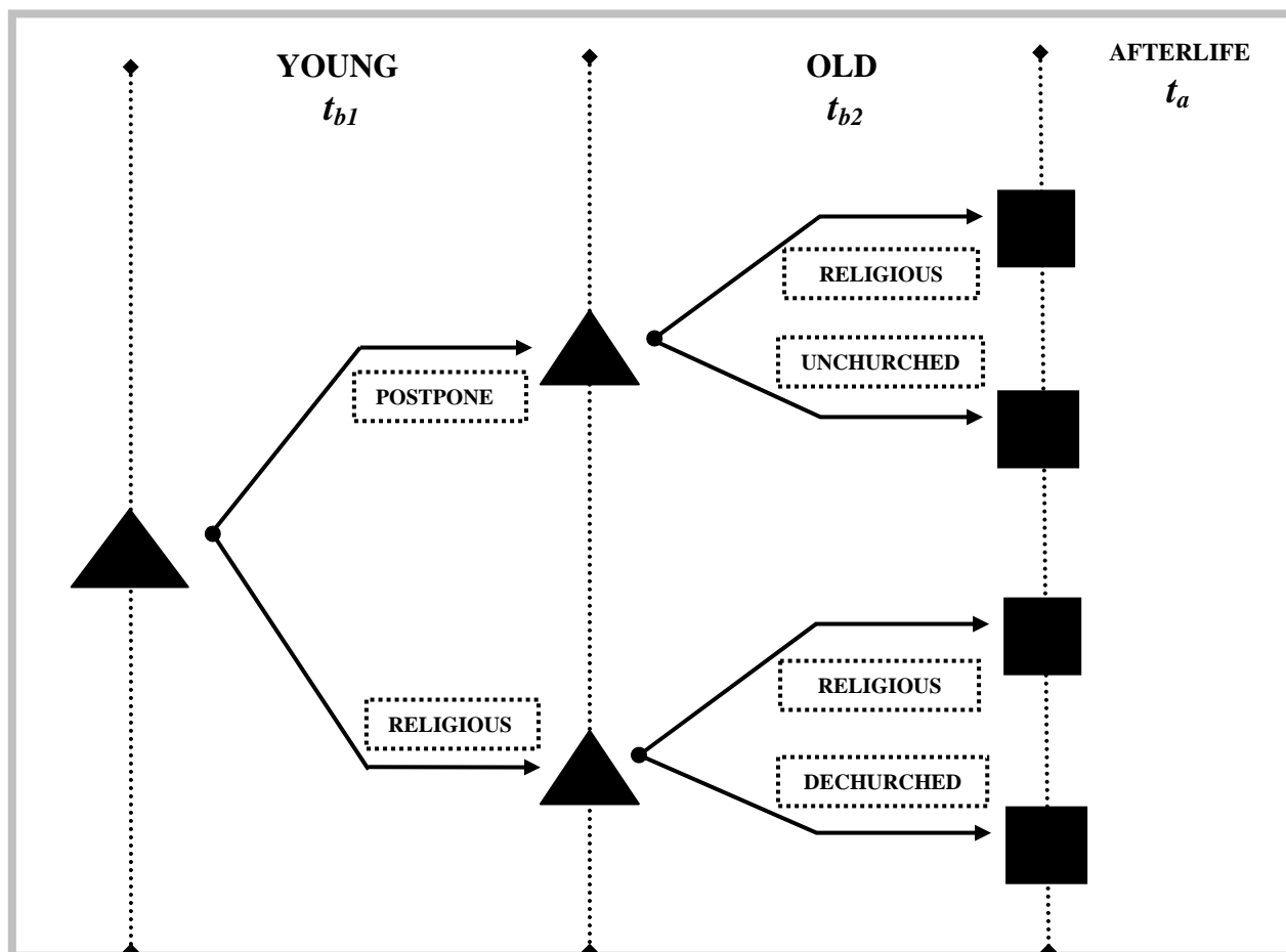
Figure 1. Decision Tree
