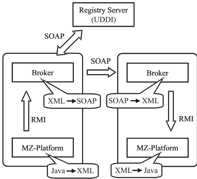
Fig. 4: Architecture of remote component
