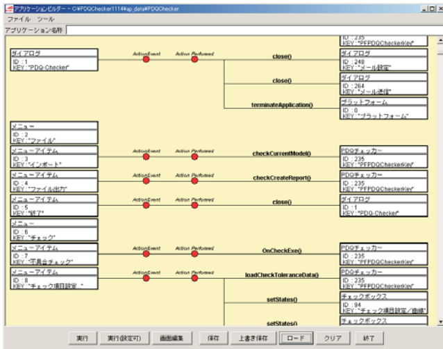
Fig. 2: Application Builder of MZ-Platform
