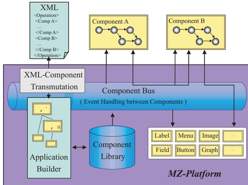
Fig. 1: Architecture of MZ-Platform
