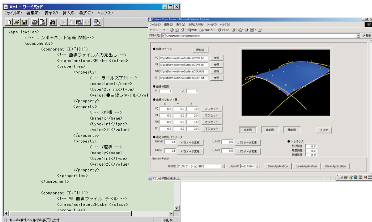
Fig. 3: Component Assembly information stored in XML format and the corresponding application
