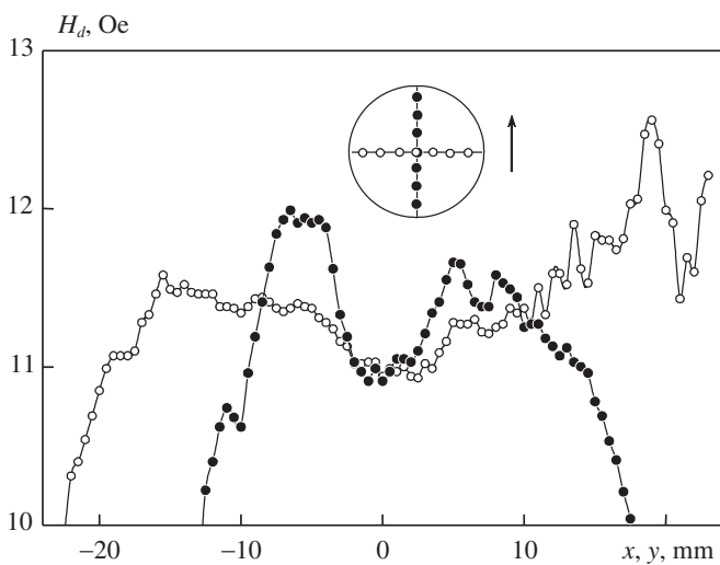
Fig. 9.: TMF magnetic reversal fields along two orthogonal directions: along the line of grinding (black points) and transversely to the line of grinding
