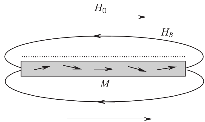
Fig. 3.: The investigated sample in a uniform magnetic field
