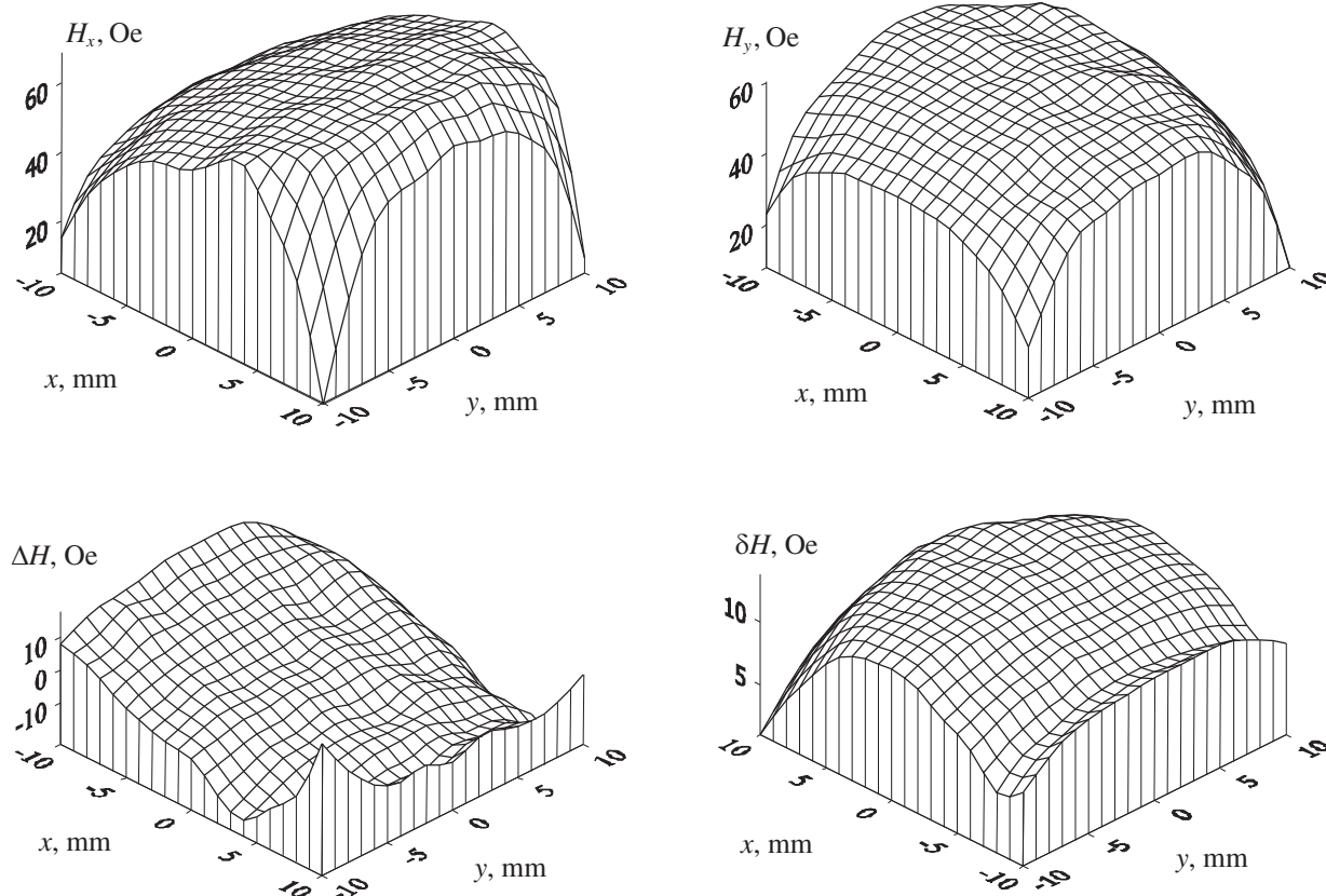
Fig. 7.: Distributions of the magnetic reversal field of TMF in the detector in the central area of a sample manufactured by one-entry grinding. H_{dy} corresponds to magnetizing along the grinding direction and H_{dx} corresponds to magnetizing in the perpendicular direction; \Delta H_d is the distribution of the difference of these fields; \delta H_d is the distribution of hysteresis.
