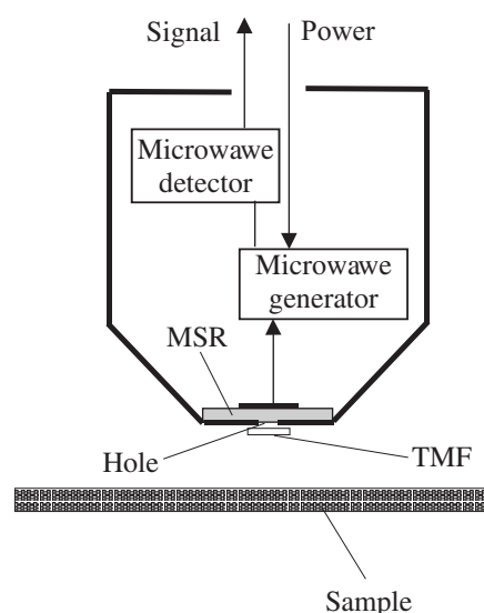
Fig. 1.: Layout of MW detector of magnetic field
