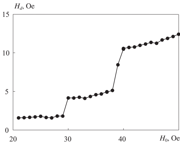
Fig. 4.: Dependence of the TMF magnetic reversal field on the value of magnetizing field applied along the direction of the sample treatment
