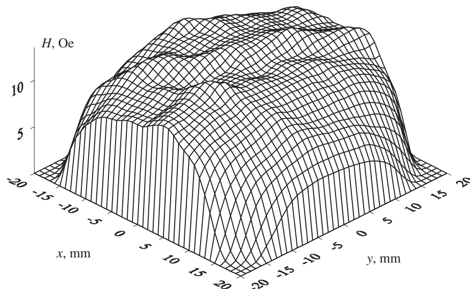
Fig. 6.: Distribution of magnetic reversal field of TMF in the detector across the surface of a sample manufactured by two-entry grinding
