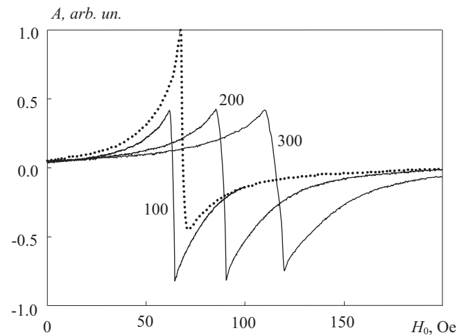
Fig. 5.: Typical FMR signals recorded with the opposite course of magnetic field sweeping from H_0 = 100, 200 and 300 Oe. Dots display the signal obtained in the direct course of sweeping.
