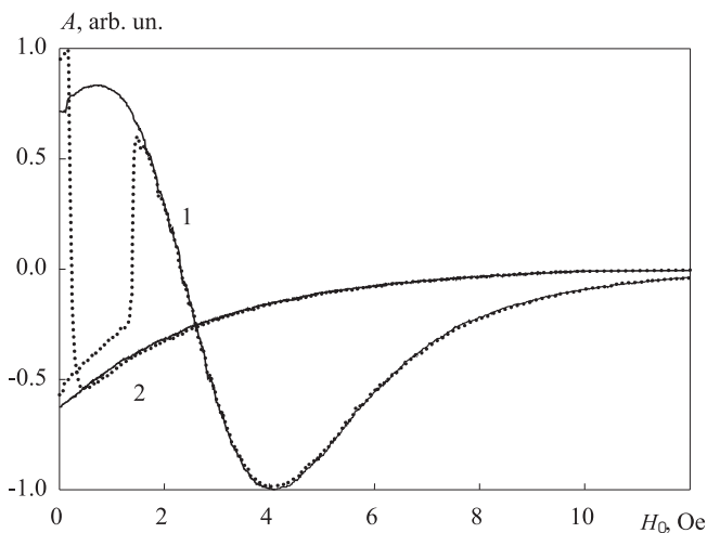
Fig. 2.: FMR curves of permalloy films having different fields of uniaxial magnetic anisotropy. 1) H_k = 1.5 Oe, 2) H_k = 4.5 Oe. Solid curves correspond to the sweeping magnetic field along the initial magnetizing, dots are the opposite sweeping.
