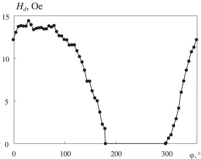
Fig. 8.: Angular dependence of the magnetic reversal field in the central area of the sample magnetized along the line of treatment
