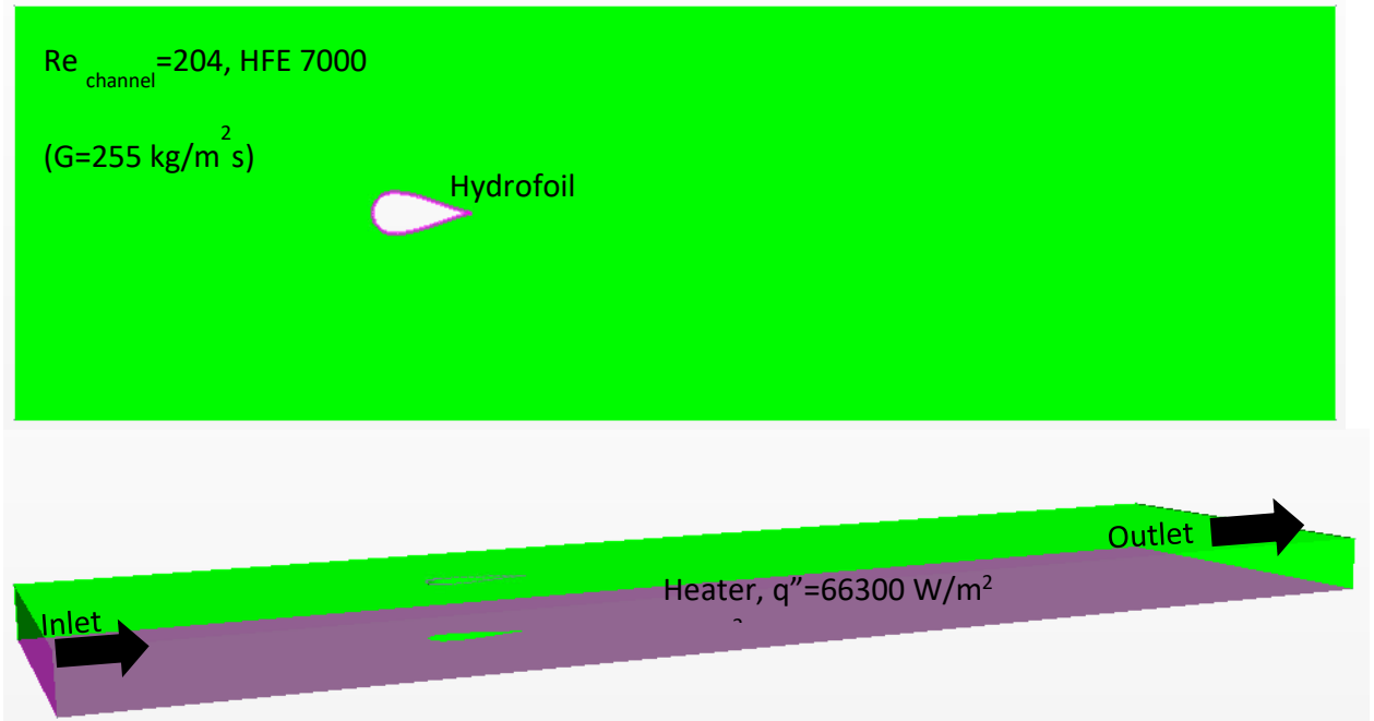
Figure 38 CFD Domain
