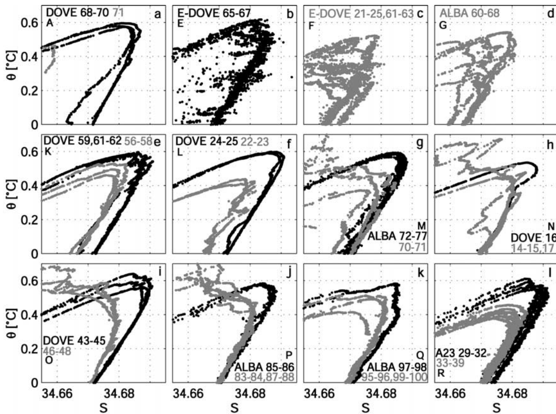
Figure 5. Potential temperature–salinity diagrams across the Weddell Front for (a) Joinville Island, east of the Antarctic peninsula; (b) Powell Basin (station 80 in gray is out of range of the plot); (c–e) Philip Passage, (f) south of the Orkney Plateau; (g) Orkney Passage; (h) north of the Orkney Plateau; (i) south of Bruce Bank; (j) Bruce Passage; (k) Discovery Passage; and (l) 31°W. CTD stations north/south of the front are marked by gray/black dots. For locations of subsections, indicated by capital letters, see Figure 1 and Table 1. DOVETAIL, E-DOVETAIL, and ALBATROSS are indicated by DOVE, E-DOVE, and ALBA, respectively.
