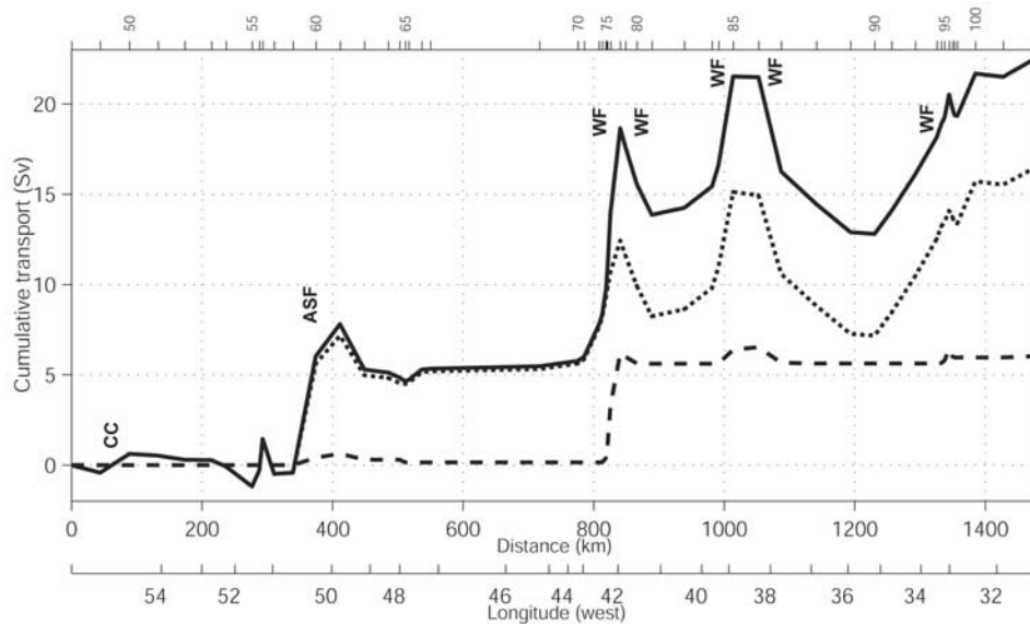
Figure 2e. Volume transports (Sv) from the ALBATROSS survey along the South Scotia Ridge, presented as cumulative transport from the tip of the Antarctic Peninsula. Geostrophic shear has been referenced to LADCP profiles as described by Naveira Garabato et al. [2002b]. All water masses (full depth water column) are depicted by the solid line; surface and intermediate water masses are depicted by the dotted line, and Weddell Sea Deep Water is depicted by the dashed line. The Antarctic Coastal Current (CC), Antarctic Slope Front (ASF), and Weddell Front (WF) crossings are marked.
