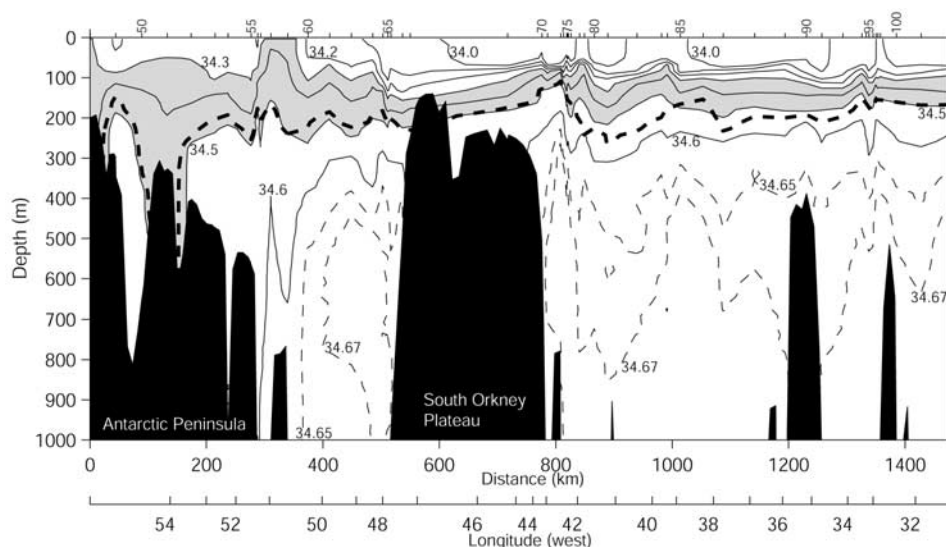
Figure 2b. As in Figure 2a but for salinity. Contour interval is 0.1, and values between 34.3 and 34.5 are shaded gray. The thin dashed contours are 34.65 and 34.67 for added detail in the Warm Deep Water.
