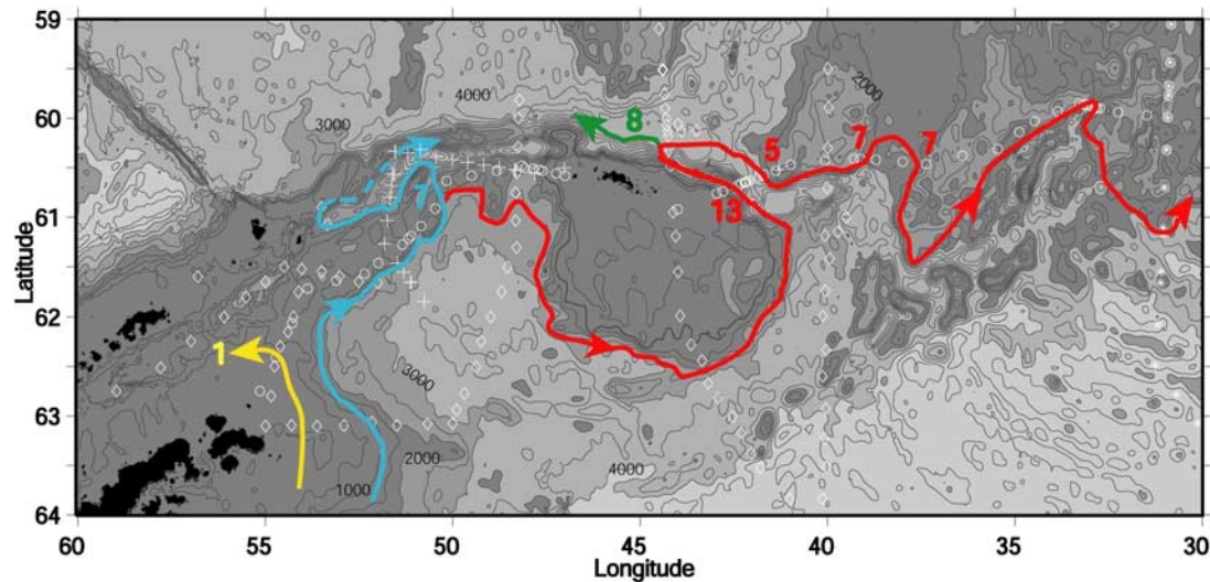
Figure 6. Schematic of the paths of fronts as deduced in this study: Antarctic Coastal Current (yellow line), Antarctic Slope Front (blue line), and Weddell Front (red line). The bathymetry and stations are shown in Figure 1. Full depth transports associated with the fronts are marked where we have measurements. The dashed blue line indicates that further observations would be needed to confirm the pathway indicated. The green line indicates the path of the Weddell Sea Deep Water that escapes westward, and the transport value given in green is for that water mass only.
