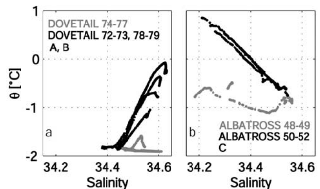
Figure 3. Potential temperature–salinity diagrams across the Antarctic Coastal Current (a) east and northeast of the Antarctic Peninsula and (b) northeast of the Antarctic Peninsula. Conductivity–temperature–depth (CTD) stations west/east of the front are marked by gray/black dots. For locations of subsections, indicated by capital letters, see Figure 1 and Table 1.
