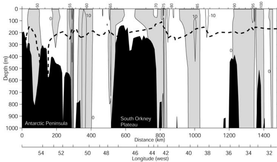
Figure 2d. As in Figure 2a but for geostrophic velocity ( \text{cm s}^{-1} ) referenced to the lowered acoustic Doppler current profiler profiles. Contour interval is 10 \text{ cm s}^{-1} , and northward (positive) values are shaded gray.
