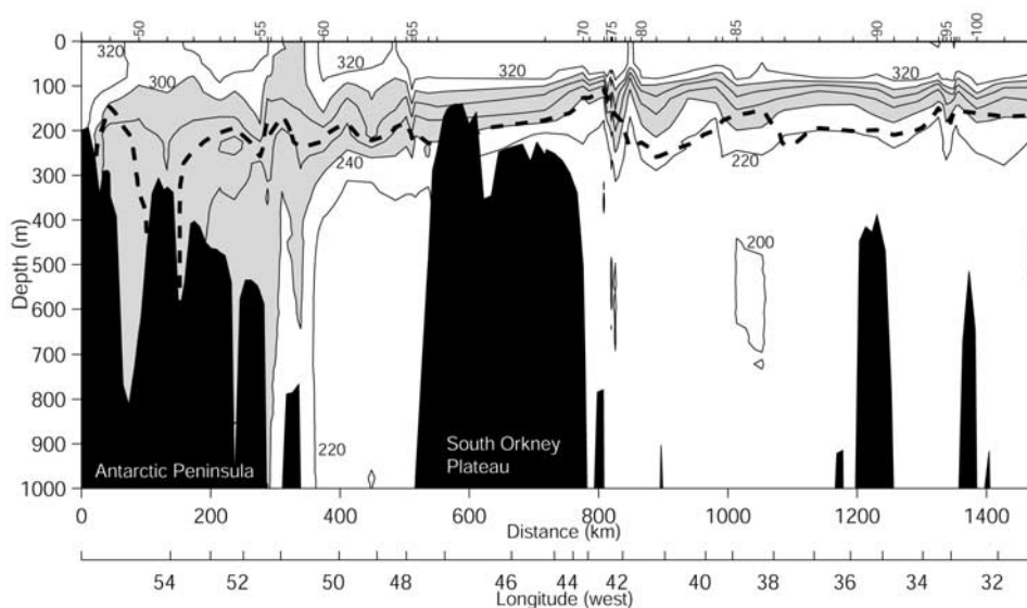
Figure 2c. As in Figure 2a but for dissolved oxygen ( \mu\text{mol kg}^{-1} ). Contour interval is 20 \mu\text{mol kg}^{-1} , and values between 240 and 300 \mu\text{mol kg}^{-1} are shaded gray.
