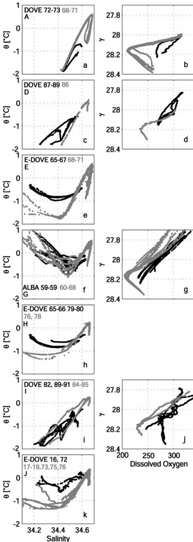
Figure 4. Diagrams of (left) potential temperature–salinity (right) and neutral density–dissolved oxygen ( \mu\text{mol kg}^{-1} ) across the Antarctic Slope Front (ASF) for (a, b) Joinville Island, east of the Antarctic Peninsula; (c–e) northwestern Powell Basin; (f–h) Philip Passage; and (i–k) Hesperides Trough. Stations in gray are to the south or east of the ASF; stations in black are to the north or west of the ASF. Dissolved oxygen data are not available for the E-DOVETAIL survey. For locations of subsections, indicated by capital letters, see Figure 1 and Table 1. DOVETAIL, E-DOVETAIL, and ALBATROSS are indicated by DOVE, E-DOVE, and ALBA, respectively.
