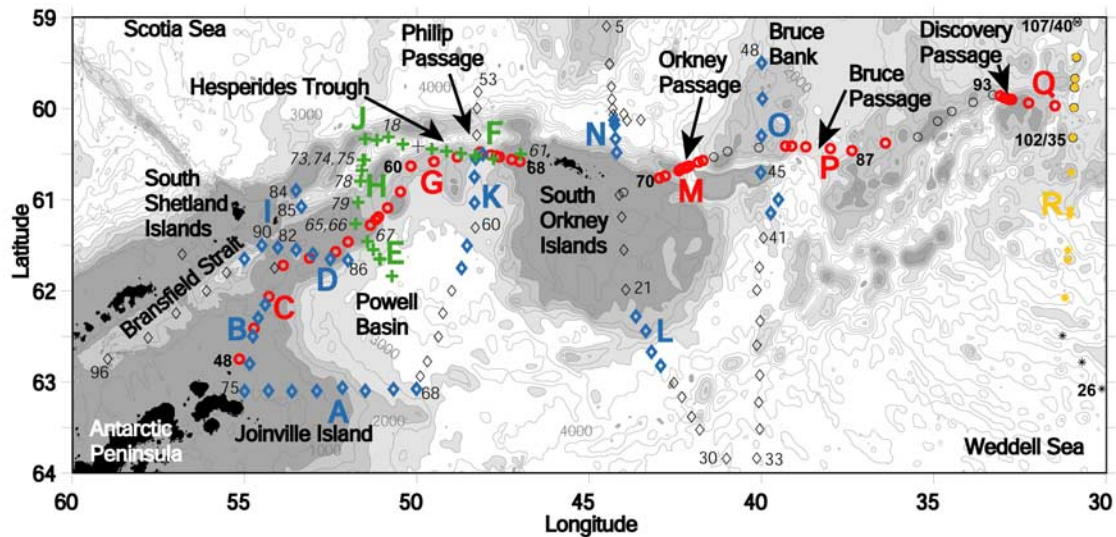
Figure 1. Bathymetry of the South Scotia Ridge region with contours every 500 m. Stations used in this study are marked: ALBATROSS stations (red circles with bold numbers), DOVETAIL stations (blue diamonds with regular numbers), E-DOVETAIL (green crosses with italic numbers), A23 stations (yellow stars with bold numbers). The same symbols in black denote stations not used for the property-property diagrams (Figures 3, 4, and 5). The color letters refer to particular subsections, detailed in Table 1.
