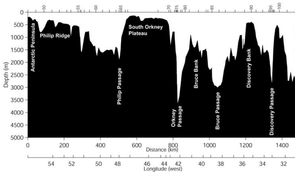
Figure 2f. Full depth bathymetry from the ALBATROSS survey along the South Scotia Ridge.
