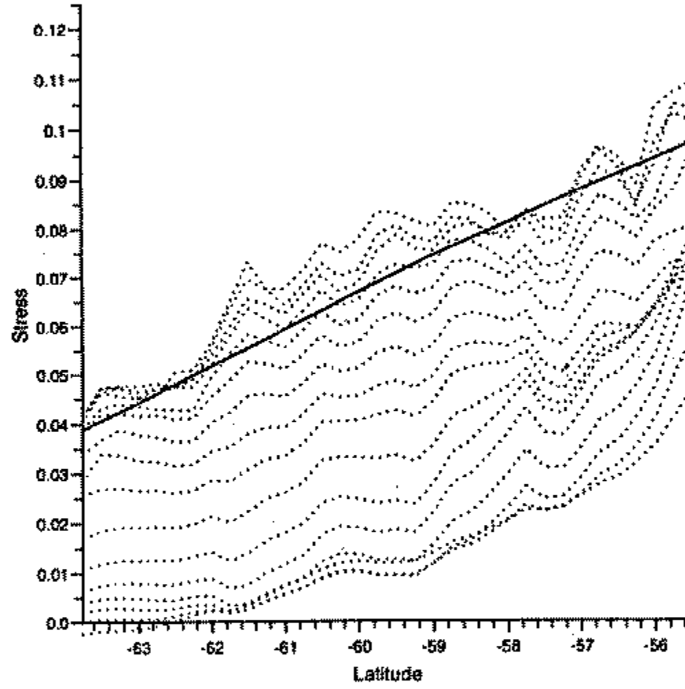
Figure 10. A comparison between the scaled eddy density flux (interfacial form stress) \rho_0 f_0 \overline{[\widehat{v} \rho]} / [\rho]_z at levels 2–17 (dotted lines) and the zonal and time averaged eastward wind stress \overline{[\tau_s^\lambda]} (solid line). The magnitude of the form stress increases with depth. Between levels 13–17 (1000–2000 m) the form stress approximately equals the wind stress. The units are \text{N m}^{-2} .
