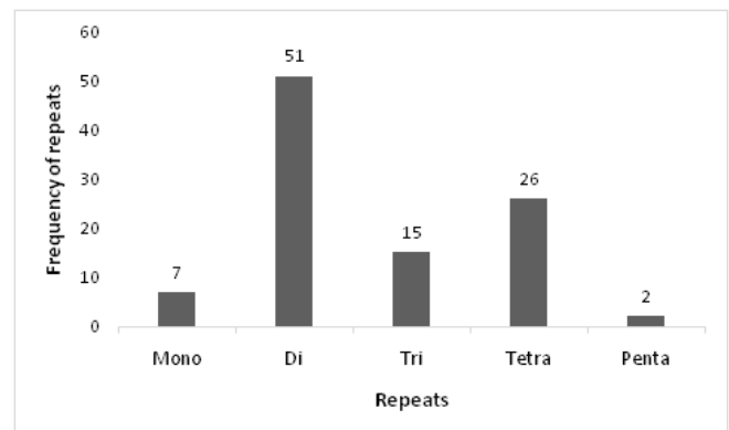
Fig. 1. Identified repeats in mitochondrial genomes of order Hypnales
