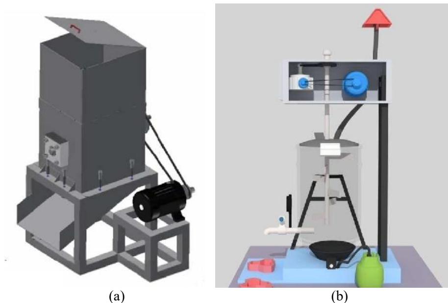
Figure 3. Handler of plastic waste for generating paving: a) plastic waste chopper; b) paving machine
