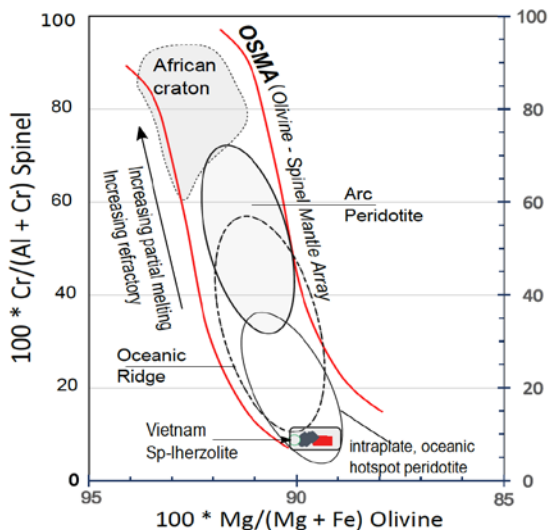
Figure 5. Olivine - Spinel Mantle Array (OSMA) showing distribution fields of peridotites from various tectonic settings. Residual peridotites produced by high degrees of partial melting are refractory (and depleted), having high Cr- numbers and forsterite contents. Redrawn after Arai (1994), data for oceanic ridges and intraplate oceanic hotspots are from Choi et al. (2005), Workman and Hart (2005) and Warren (2016)
