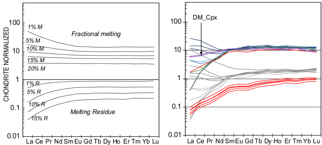
Figure 8a, b. Chondrite normalized computed rare earth element abundance produced by fractional melting (Eq. 1); A%M and A%R: rare earth element composition of melt (M) or residue (R) produced by A melting degree (8a, left); rare earth element chondrite normalized distribution pattern of Nghia Dan clinopyroxene (thick, red line) and corresponding residual parental peridotite (thin, red lines) according to different mineral constituents (8b, right). Shown for comparison are clinopyroxene separate and their residual peridotite from Dat Do (Ba Ria- Vung Tau), and clinopyroxene (DM_Cpx) separated from the representative depleted mantle peridotite (Computing template is after Workman and Hart, 2005; Warren, 2016). Normalizing data are after Anders and Grevesse (1989)
