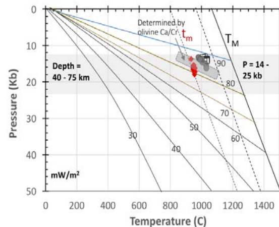
Figure 10. A geotherm for Nghia Dan determined by spinel lherzolite (thick dashed line) using two-pyroxene geothermobarometers by Putirka et al. (1996, 2003) and Putirka (2008, 2017). Thin solid lines are model conductive geotherms of continental areas with surface heat flows from 30 to 90mW/m 2 (Pollack and Chapman, 1977). Thin dashed line ( t_m ) thermally normal mantle adiabatic line ca. 1280°C, Thick continuous line ( T_M ) continuous line, elevated temperature adiabatic, ca. >1380°C (Hoang unpublished. Shown for comparison are mantle xenoliths from Pleiku: red filled diamonds, Tro islet (Ile des Cendres): white filled square (Malinovsky and Rashidov, 2015), Western Highlands and Southeastern region of Vietnam: filled rectangle (Hoang unpublished data)
