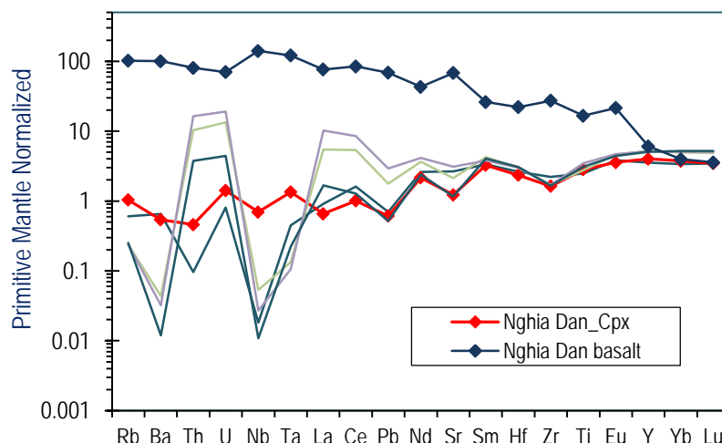
Figure 6. Trace element primitive mantle normalization of Nghia Dan clinopyroxene separate showing relatively smooth trend from moderately immobile to highly mobile elements (normalizing data are after Sun and McDonough, 1989). Shown are data for the host alkaline basalt and mantle xenolith- separated clinopyroxenes from Dat Do (Ba Ria - Vung Tau) for comparison. See text for details
