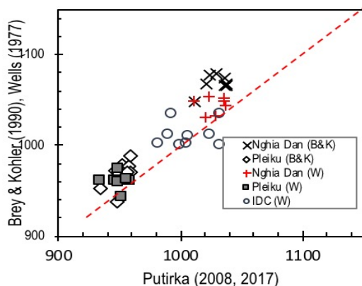
← Figure 9. Plots of temperature estimates for equilibrium two-pyroxenes in Nghia Dan mantle xenoliths using geothermometers of Wells (1977), Brey and Köhler (1990) versus Putirka (2008, 2017). Data for Pleiku (Western Highlands) and Tro Islet (Ile des Cendres, East Vietnam Sea) mantle xenoliths (Hoang unpublished data) are shown for reference
