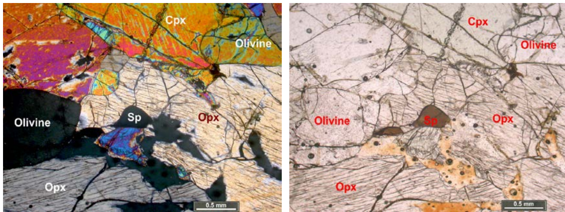
Figure 4. Photomicrograph of a spinel-lherzolite xenolith with xenogranular texture recovered at Mt. Ke Lui (Nghia My) showing a mineral assemblage comprising olivine, orthopyroxene, clinopyroxene and spinel: cross polarized (left), plain polarized (right)
