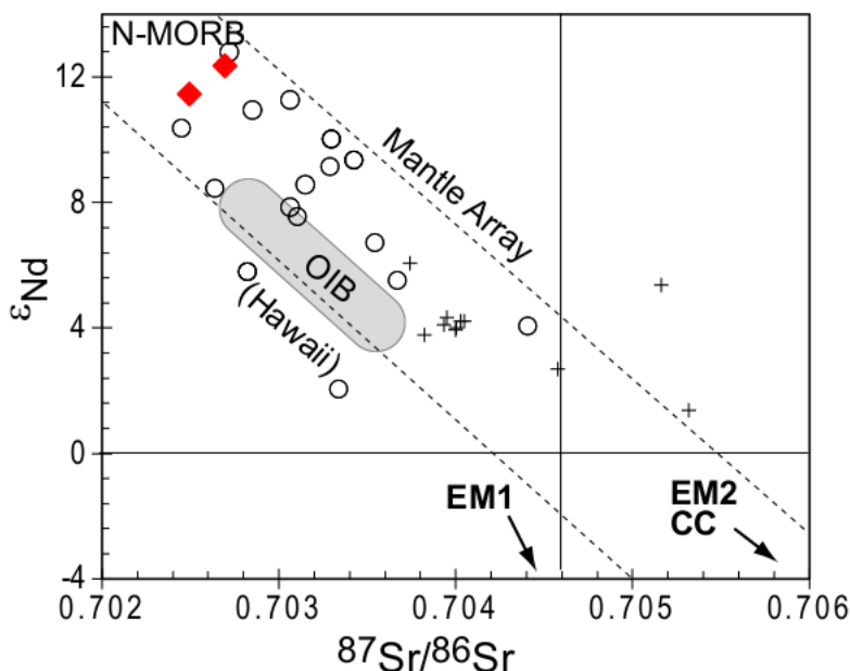
Figure 7. Plots of ^{87}\text{Sr}/^{86}\text{Sr} versus \epsilon_{\text{Nd}} [ = (^{143}\text{Nd}/^{144}\text{Nd}_m/0.512638)-1 \times 10000 ] of Vietnam alkaline basalt-borne mantle xenolith separated clinopyroxenes (empty circles; Hoang unpublished data) including Nghia Dan (red filled diamond) (Table 2) and host basalts (cross). Shown are fields of Depleted Mid-Ocean Ridge Basalt Mantle (N-MORB), Enriched Mantle type 1 and 2 (EM1 and EM2) (after Zindler and Hart, 1986); field of continental crust (CC) (after Taylor and McLennan, 1981) and Oceanic Island basalt (OIB Hawaii, after Norman and Garcia, 1999) for reference
