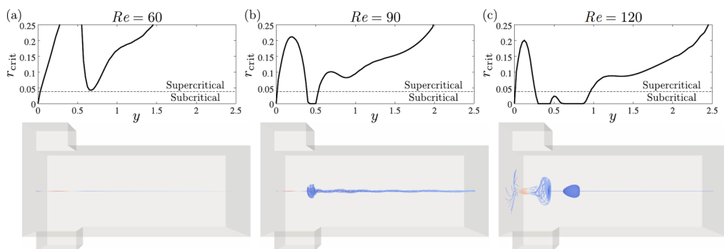
FIG. 8. Numerical results computing the criticality of our flows using the approach presented by Ruith et al. [6]. As can be seen, the appearance of a pocket of subcriticality corresponds to the appearance of vortex breakdown. Results correspond to (a) Re = 60 , (b) Re = 90 , and (c) Re = 120 , for which we expect zero, one, and two regions of vortex breakdown in the flow. In each case, the axial locations where pockets of subcriticality appear correspond precisely with the locations of vortex breakdown.
