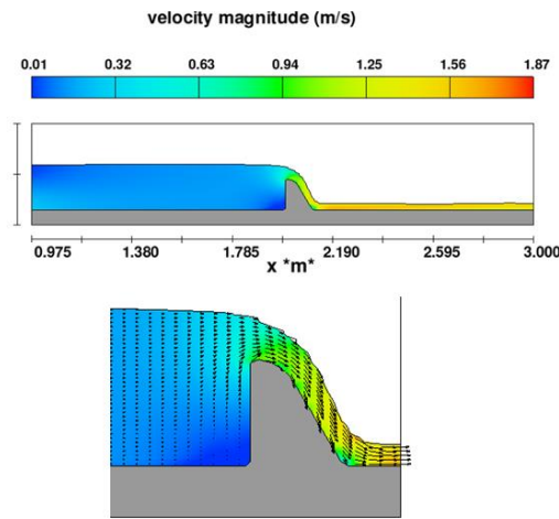
Figure 13. The changes of flow velocity on circular crested weirs in group F
