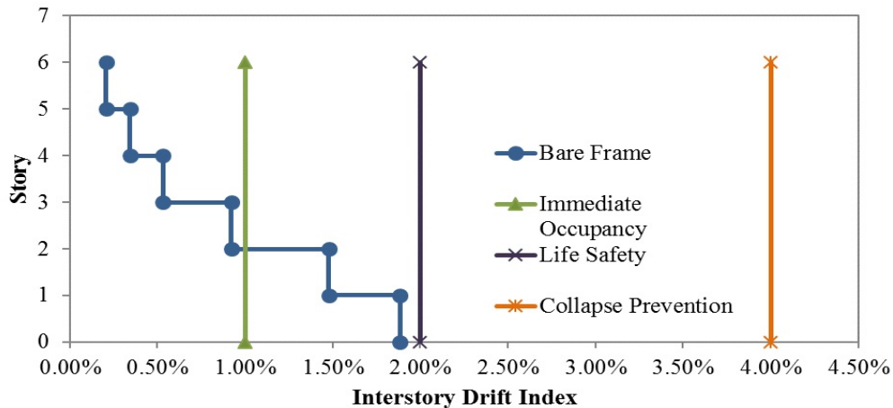
Figure 12. Interstory drift index of the RC frame
