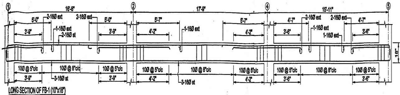
(c) Long section of floor beam, FB1
