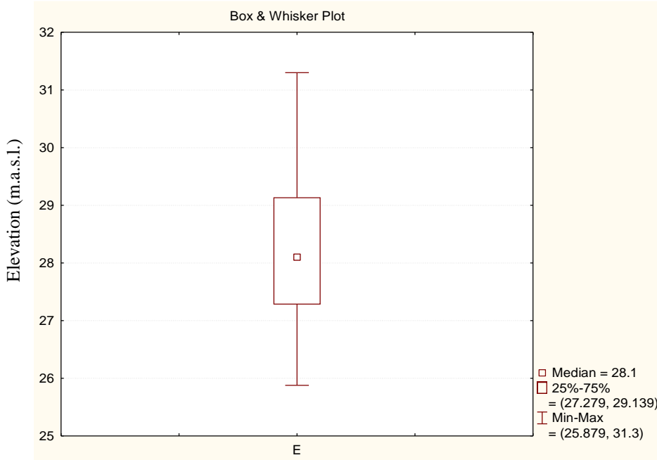
Figure 6(a). Box & Whisker test for elevation (E(m.a.s.l.))
