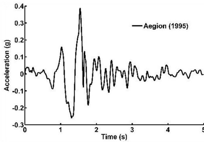
Figure 7. Ground motion time history used in the verification analysis
