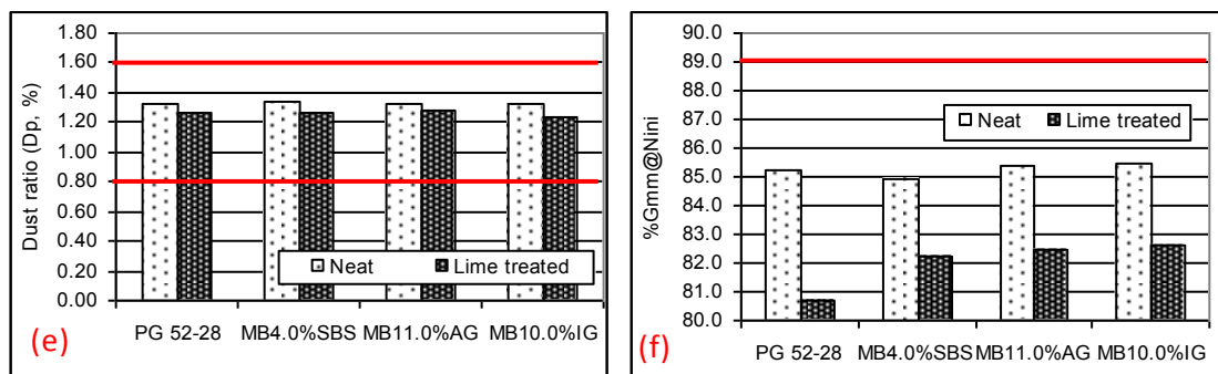
Figure 4. Volumetric properties of mixtures
