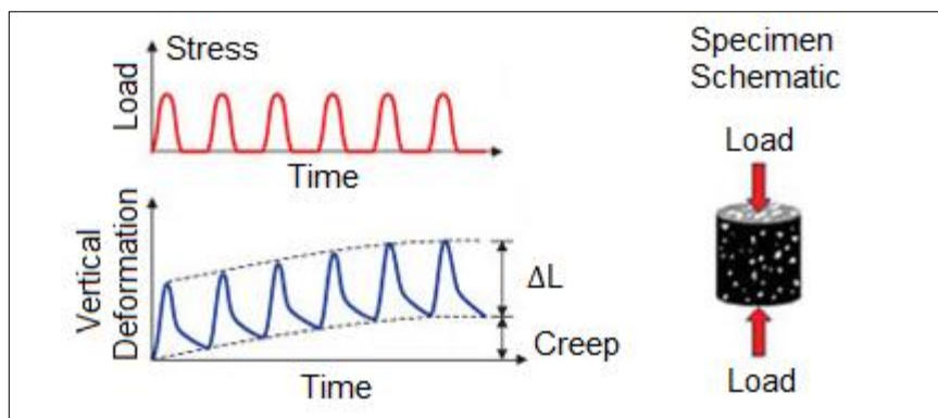
Figure 5. Relationships between the Load-Time and the Deformation-Time [27]
