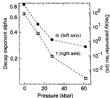
FIG. 2. Variation with pressure of the decay parameters \alpha and \tau for the fits shown in Fig. 1.
