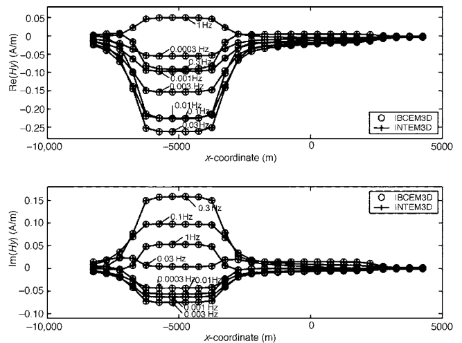
Figure 11. Model 2. Plots of the real and imaginary parts of the sum of magnetic fields H_y^{\Delta\sigma_p} and H_y^{\Delta\sigma_s} along the x -directed profile at y = -1250 m. The solid lines represent the results obtained by INTEM3D; the circles show the data computed by IBCEM3D.
