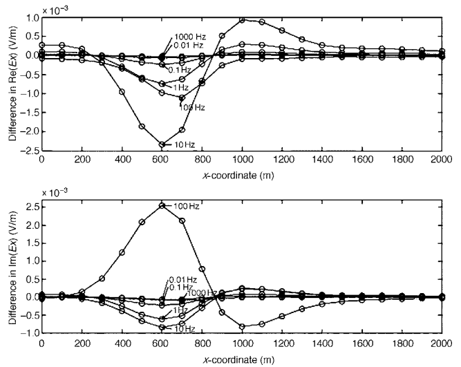
Figure 5. Model 1. Plots of the differences (errors) between the results obtained by two algorithms, INTEM3D and IBCEM3D, for the real and imaginary parts of the sum of electric fields E_x^{\Delta\sigma_b} and E_x^{\Delta\sigma_a} along an x -directed profile at y = 0 .
