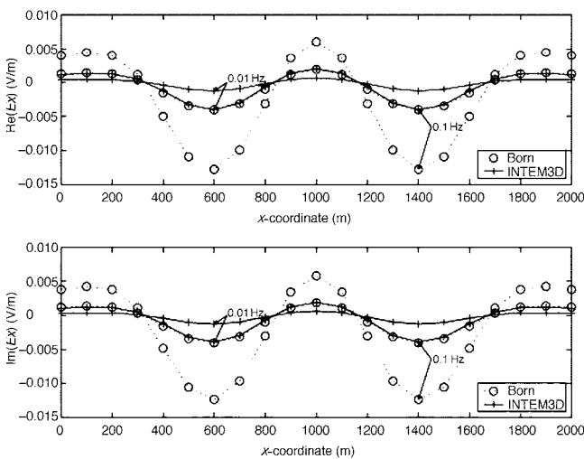
Figure 7. Plots of the real and imaginary parts of the sum of electric fields E_x^{\Delta\sigma} and E_x^{\Delta\sigma} along the x -directed profile at y = 0 . The solid lines represent the results obtained by the conventional IE method (INTEM3D); the circles show the data computed using Born approximation.
