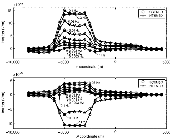
Figure 13. Model 3. Plots of the real and imaginary parts of the sum of electric fields E_x^{\Delta\sigma_n} and E_x^{\Delta\sigma_n} along the x -directed profile at y = 1250 m. The solid lines represent the results obtained by INTEM3D; the circles show the data computed by IBCEM3D.
