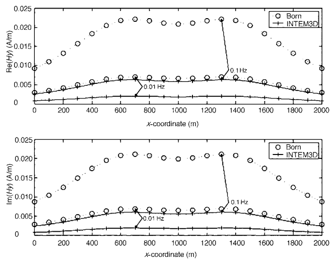
Figure 8. Plots of the real and imaginary parts of the sum of magnetic fields H_y^{\Delta\sigma} and H_y^{\Delta\sigma} along the x -directed profile at y = 0 calculated for Model 1. The solid lines represent the results obtained by INTEM3D; the circles show the data computed by Born approximation.
