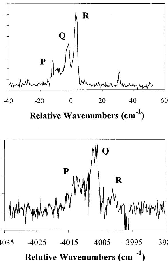
FIG. 2. Rotational band contour obtained by dispersed fluorescence of the 0-0 band of the [18.6] \Omega'=1 \rightarrow X^3\Sigma_{0+}^- system of MoC (upper panel), compared to the 0-0 band of the [18.6] \Omega'=1 \rightarrow [4.0]^3\Delta_2 system (lower panel).
