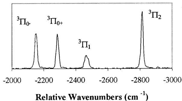
FIG. 5. Dispersed fluorescence of PdC obtained following excitation of the [17.9]^3\Sigma_1^+ \leftarrow X^1\Sigma^+ , 0-0 band. Emission to the \Omega=0^-, 0^+, 1, and 2 substates of the [...]12\sigma^16\pi^1, ^3\Pi state is observed. The ^3\Pi_1 substate is accessed via collisional deactivation of the ^3\Sigma_1^+ state to the ^3\Sigma^+(0^-) state, which lies 16.5\text{ cm}^{-1} lower in energy.
