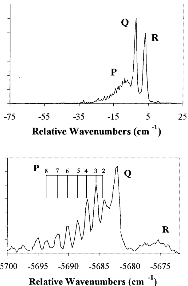
FIG. 3. Rotational band contour obtained by dispersed fluorescence of the 0-0 band of the [18.1] ^1\Pi_1 \rightarrow X^1\Sigma^+ system of RuC (upper panel), compared to the 0-0 band of the [18.1] ^1\Pi_1 \rightarrow [5.7]^1\Delta_2 system (lower panel). Rotational lines of the P-branch are partially resolved, giving B_0(^1\Delta_2) = 0.5964 \pm 0.0004 cm -1 .
