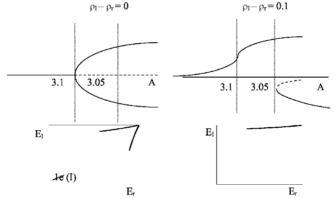
FIG. 5. The effect of an imperfect symmetry in the problem is illustrated in the case of the transition from a solution with symmetry 1e to the pair of conjugate solutions of symmetry type 1\ell in the symmetric case (left panel) and in the imperfect case (right panel). In an open range of parameters, only one of the conjugate solutions survives.
