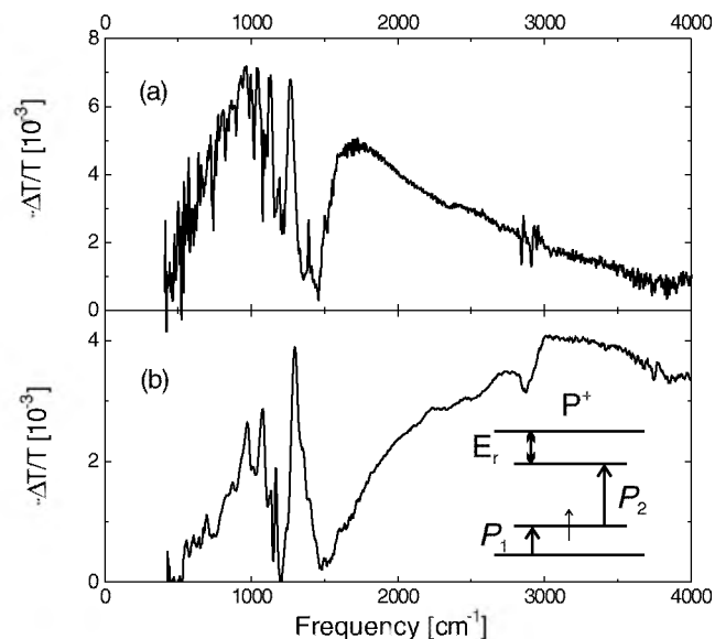
FIG. 1. PA spectra in the mid-IR range for films of RR-P3HT (a) and RR-P3AT with a long attached alkyl side group (b). The inset shows schematically the two polaron levels in the gap and associated optical transitions P_1 and P_2 ; the polaron relaxation energy E_r is also defined ( E_r \approx P_1 ).
