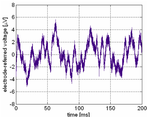
Fig. 10. Measured input-referred noise for f_H = 100 Hz.
