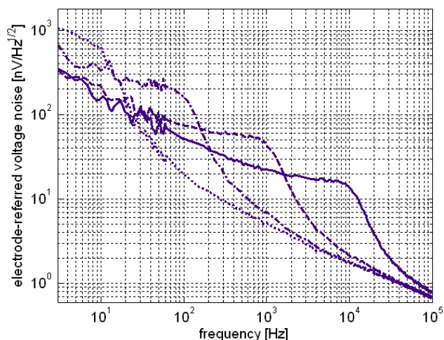
Fig. 11. Input-referred noise spectra for f_H = 10 Hz (dot), f_H = 100 Hz (dash-dot), f_H = 1 kHz (dash), and f_H = 10 kHz (solid).
