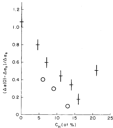
FIG. 3. Dependence of the relative height of the induced absorption peak at t=0 on hydrogen concentration. Crosses, a -Si:H; circles, a -Si:H:F. ( C_F \approx 14 at.%) T = 300 K.
