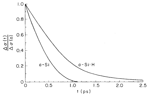
FIG. 4. Time dependence of the normalized hot-carrier absorption cross section \Delta\sigma = \sigma - \sigma_s in a -Si and a -Si:H at 80 K.
