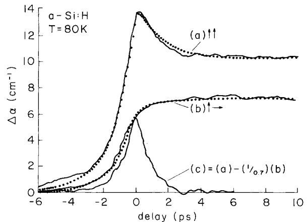
FIG. 2. Same as Fig. 1, but for a -Si:H with hydrogen concentration C_H=10\% .
