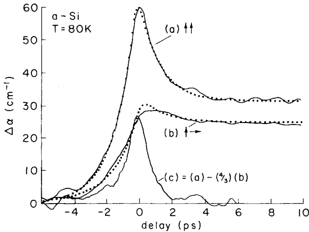
FIG. 1. Time dependence of the photoinduced absorption in a -Si for \parallel and \perp polarizations. Solid curves, experimental; dotted curves, calculated.
