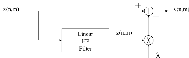
Fig. 1. Unsharp masking for contrast enhancement.
