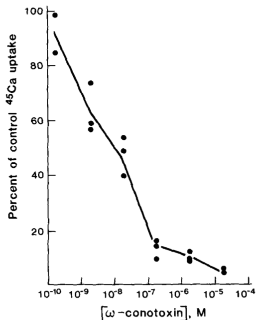
FIG. 3. Concentration dependence of \omega -conotoxin inhibition of 45 Ca uptake by chick brain synaptosomes. 45 Ca uptake was measured as described under "Experimental Procedures." The synaptosomes were preincubated with \omega -conotoxin at the concentrations indicated for 30 min before 45 Ca uptake was measured. In this experiment, the actual values for 45 Ca uptake were: high K control, 6000 cpm; low K control 1280 cpm. Thus, the difference between these two values, 4720 cpm was set as 100% of voltage activated 45 Ca uptake. Each experimental point for 45 Ca uptake in the presence of \omega -conotoxin with the low K control (1280 cpm) subtracted out is shown by the circles; the line is drawn to the average of these points at each \omega -conotoxin concentration.
