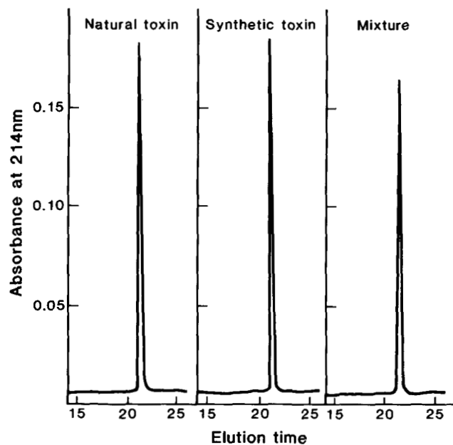
FIG. 2. HPLC comparison of synthetic and natural \omega -conotoxin GVIA. Synthetic and natural \omega -conotoxin GVIA (~1 nmol each), as well as an equimolar mixture (~0.45 nmol each) were chromatographed at 25 °C on a Vydac C 18 analytical column. The peptides were eluted using 0.1% trifluoroacetic acid as solvent, applying a linear gradient from 9–28% (v/v) acetonitrile at a flow rate of 1 ml/min.
