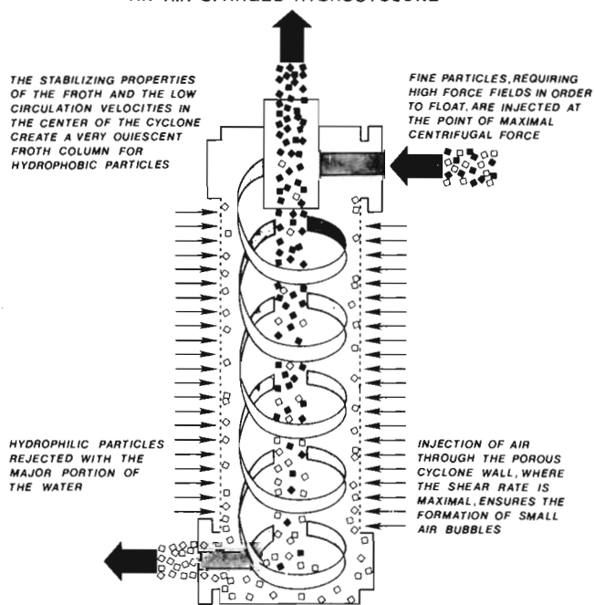
Fig. 5—Schematic drawing of the preferred air sparged hydrocyclone design.
