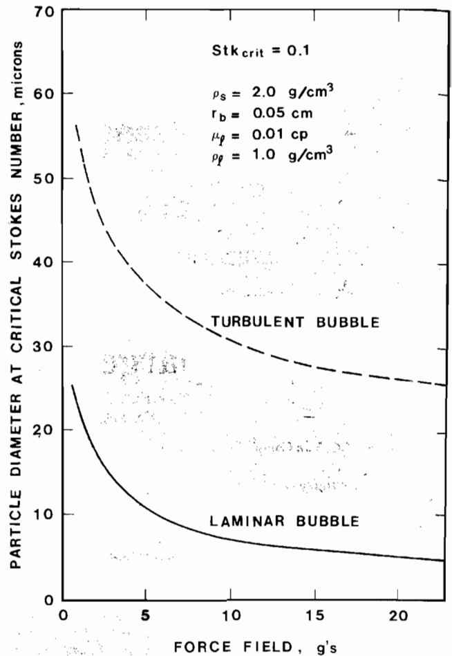
Fig. 2—Minimum particle diameter for inertial impaction as a function of the force field magnitude assuming a critical Stokes number of 0.1 (Miller, Kinneberg, and Van Camp, 1982).
