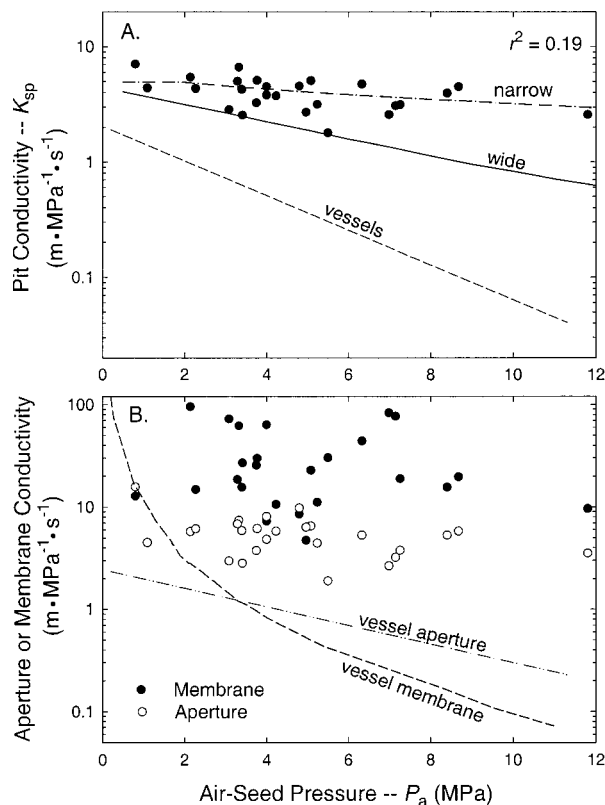
Fig. 8. (A) Pit conductivity per membrane area (pit K_{sp} ) vs. air-seed pressure ( P_a ) for root and stem xylem samples in the data set (symbols; overall r^2 = 0.19 ). Dash-dotted line is for tracheids of the narrowest diameter in the data set ( D_c = 7.3 \mu\text{m} ; D_m = 6.2 ; D_a = 1.9 ; D_t = 3.0 \mu\text{m} ). Solid line is for tracheids of the widest diameter ( D_c = 51 \mu\text{m} ; D_m = 19.8 ; D_a = 4.8 ; D_t = 9.0 \mu\text{m} ). Dashed line is correlation for vessel data from Sperry and Hacke (2004). (B) Aperture (open symbols) or membrane (solid symbols) conductivity per membrane area vs. air-seed pressure for same xylem samples from (A). Dotted line shows vessel aperture conductivities and dashed line shows vessel membrane conductivities from Sperry and Hacke (2004).
