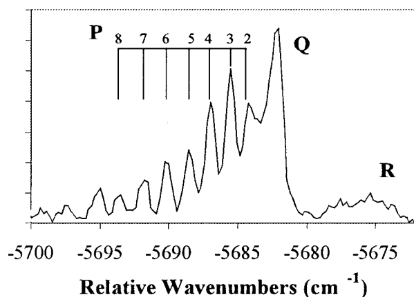
FIG. 3. Rotational band contour obtained by dispersed fluorescence of the 0-0 band of the [18.1] ^1\Pi_1 \rightarrow X^1\Sigma^+ system of RuC (upper panel), compared to the 0-0 band of the [18.1] ^1\Pi_1 \rightarrow [5.7]^1\Delta_2 system (lower panel). Rotational lines of the P-branch are partially resolved, giving B_0(^1\Delta_2) = 0.5964 \pm 0.0004 cm -1 .
