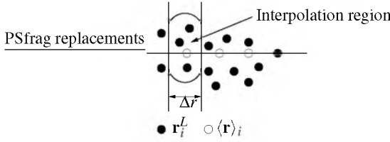
Figure 1: Directional local grid. A one-dimensional grid is created in the particle's streamline direction. The quantities are only interpolated in the cut disk area. (After Heo et al. 12 )
