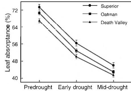
Fig. 2. Mean leaf absorbance at different drought stages for three populations of Encelia farinosa growing under common environment conditions. Leaf absorbance values differed among populations ( P < 0.001 ) and among drought stages ( P < 0.001 ), but the population by drought stage interaction was not significant ( P = 0.06 ), indicating that the slopes of response to drought were similar among populations.
