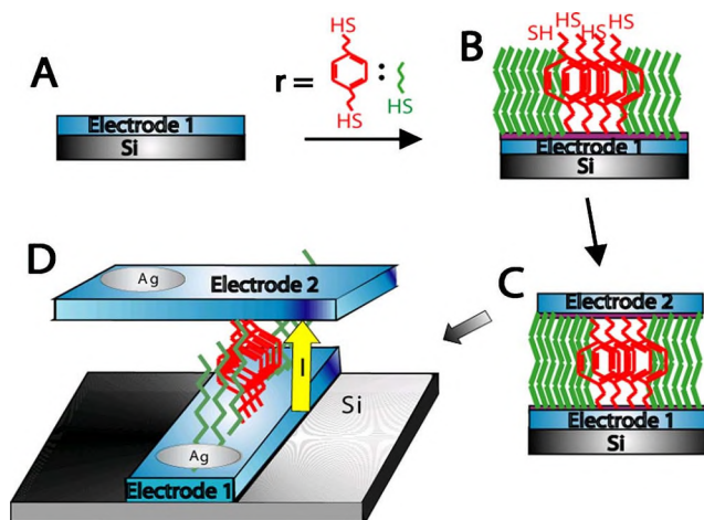
FIG. 1. (Color online) The fabrication process (schematic) of SAM solid state mixture diodes at large ratio, r of molecular wires (Me-BDT in red) to molecular insulators (PT in green) for transport studies. (a) Evaporation of the base electrode; (b) SAM growth of the appropriate solid state mixture on the bottom electrode; (c) evaporation of the upper electrode; (d) I - V measurement setup.
