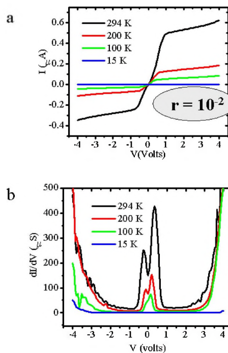
FIG. 5. (Color online) Electrical transport measurements of SAM diodes devices with r=10^{-2} at various temperatures showing Me-BDT aggregates behavior. (a) I - V characteristics; (b) differential conductance spectrum obtained from (a).
