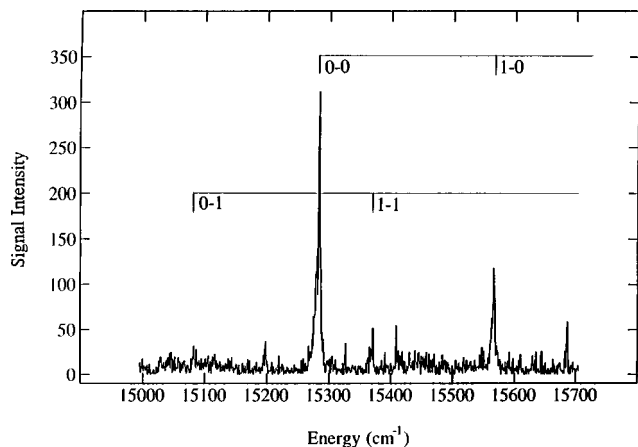
FIG. 1. A low resolution scan of the [15.3] 2\Sigma^+ \leftarrow X 2\Sigma^+ band system of ^7\text{Li } ^{40}\text{Ca} , collected using DCM dye laser radiation for excitation and the second harmonic of this radiation for photoionization. The identification of the 1-1 and 0-1 bands in this spectrum would have been impossible without the knowledge of \Delta G''_{1/2} obtained from the other band systems.
