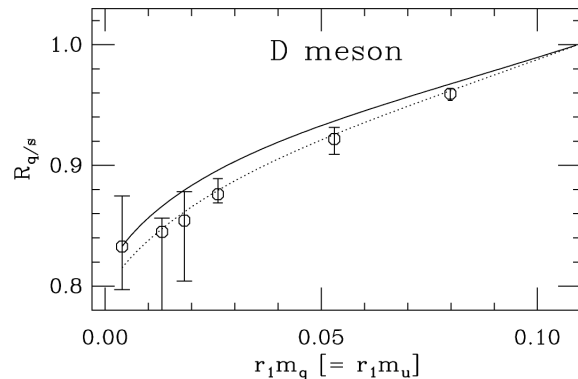
Figure 1. The chiral extrapolation of the ratio f_D\sqrt{m_D}/f_{D_s}\sqrt{m_{D_s}} . The ratio is determined by the solid curve where staggering effects have been removed. The dashed curve includes these discretization effects.
