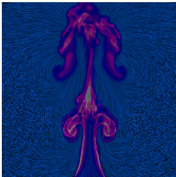
Figure 4: JP8 dataset.
