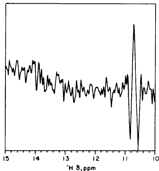
FIG. 6. A ^1\text{H} - ^{15}\text{N} FINDS spectrum at 15 °C for E. coli tRNA Met . tRNA Met from E. coli grown on [1- ^{15}\text{N} ]uracil. The sample was dissolved in 10 mM cacodylate buffer, pH 7.0, containing 50 mM sodium chloride, 10 mM magnesium chloride, 1 mM EDTA, and 8% (v/v) deuterium oxide. A total of 2400 scans was accumulated with broadband irradiation of ^{15}\text{N} chemical shift (on-resonance) and 1000-Hz downfield (off-resonance) on alternate scans.
