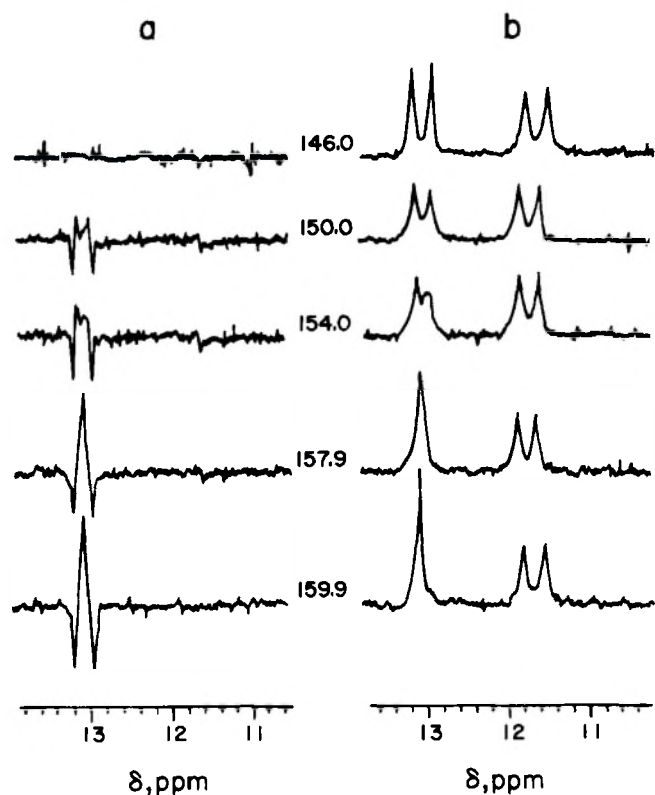
FIG. 2. Fourier internuclear difference spectroscopy (FINDS) and 1 H spectra of [1,3- 15 N 2 ]5-(2',5',8'-trioxadecyl)uracil. A 1:1 mixture of [1,3- 15 N 2 ]5-(2',5',8'-trioxadecyl)uracil and 2',3'-O-isopropylidene-5'-O-acetyl adenosine in chloroform-d at 25 °C, 0.2 M total nucleoside concentration. FINDS is shown in part a and normal 1 H spectra in part b. Sixteen scans were acquired with irradiation of 15 N at the chemical shifts indicated between the FINDS and 1 H spectra (on-resonance) or at 1000 Hz downfield from the indicated chemical shift (off resonance).
