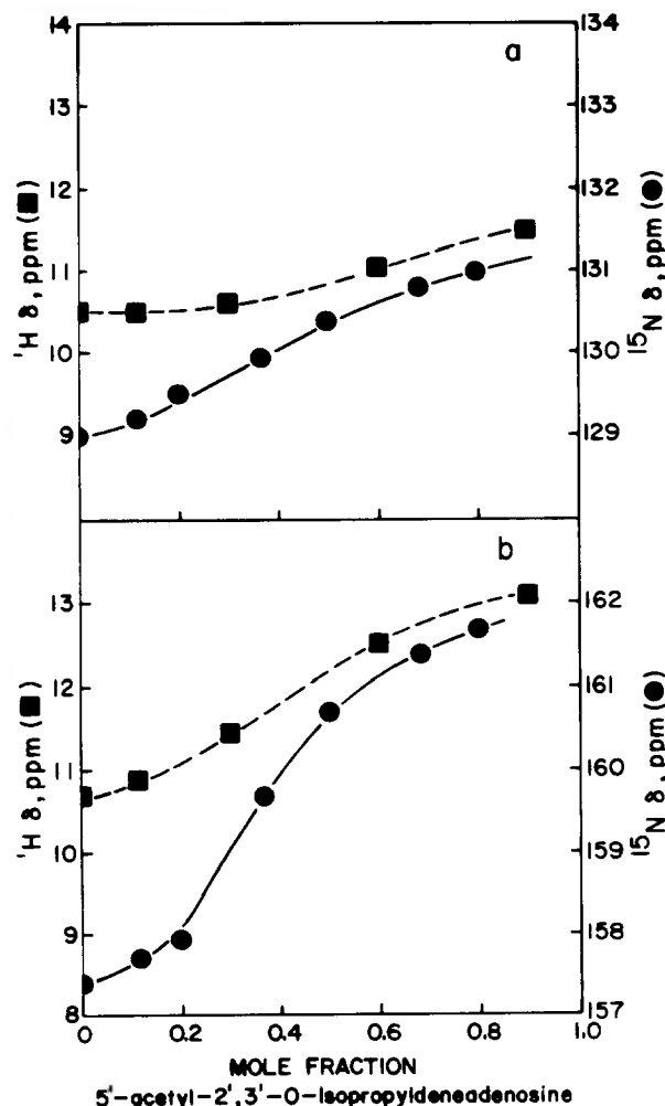
FIG. 5. ^1\text{H} and ^{15}\text{N} chemical shifts for solutions of [1,3- ^{15}\text{N}_2 ]5-(2',5',8'-trioxadecyl)uracil and 5'-acetyl-2',3'- O -isopropylidene adenosine. ^1\text{H} (■) and ^{15}\text{N} (●) chemical shifts measured with solutions 0.2 M in total nucleoside at 26 °C. Part a, N1 imino unit; part b, N3 imino unit.
