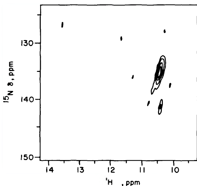
FIG. 8. A contour map of a ^1\text{H} - ^{15}\text{N} FES spectrum at 15^\circ\text{C} for E. coli \text{tRNA}^{\text{Glu}} . \text{tRNA}^{\text{Glu}} from E. coli grown on [1\text{-}^{15}\text{N}]\text{uracil} . The sample was dissolved in 10 mM cacodylate buffer, pH 7.0, containing 100 mM sodium chloride, 15 mM magnesium chloride, 1 mM EDTA, and 8% (v/v) deuterium oxide. A total of 1600 \times 20 scans was acquired with ^{15}\text{N} decoupling. The t_1 dimension was zero-filled to 128 data points and a total of 2000 \times 128 points was multiplied by an exponential factor corresponding to 15 Hz of line broadening in each dimension and transformed. The absolute value spectrum is plotted.
