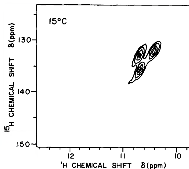
FIG. 10. A contour map of a ^1\text{H} - ^{15}\text{N} FES spectrum at 15 °C for E. coli tRNA Phe . tRNA Phe from E. coli grown on [ ^{15}\text{N} ]uracil. The sample was prepared as described in the legend to Fig. 8. A total of 800 × 24 scans was collected with ^{15}\text{N} decoupling. The t_1 dimension was zero-filled to 128 data points, and a total of 2000 × 128 points was multiplied by an exponential factor corresponding to 15 Hz of line broadening in each dimension and transformed. The absolute value spectrum is plotted.
