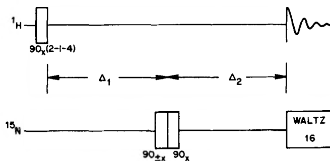
FIG. 3. Pulse sequence for J -modulated internuclear difference spectroscopy.
