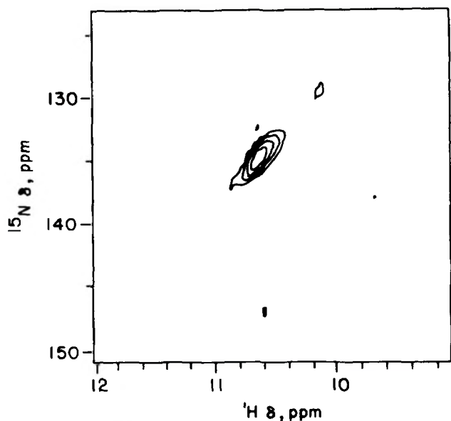
FIG. 7. A contour map of a ^1\text{H} - ^{15}\text{N} FES spectrum at 15^\circ\text{C} for E. coli \text{tRNA}^{\text{Met}} . \text{tRNA}^{\text{Met}} from E. coli grown on [1\text{-}^{15}\text{N}]\text{uracil} . The sample was prepared as described in the legend to Fig. 5. A total of 1000 \times 24 scans was acquired with ^{15}\text{N} decoupling. The t_1 dimension was zero-filled to 128 data points and a total of 1000 \times 128 points was multiplied by an exponential factor corresponding to 15 Hz of line broadening in each dimension and transformed. The absolute value of the spectrum is plotted.
