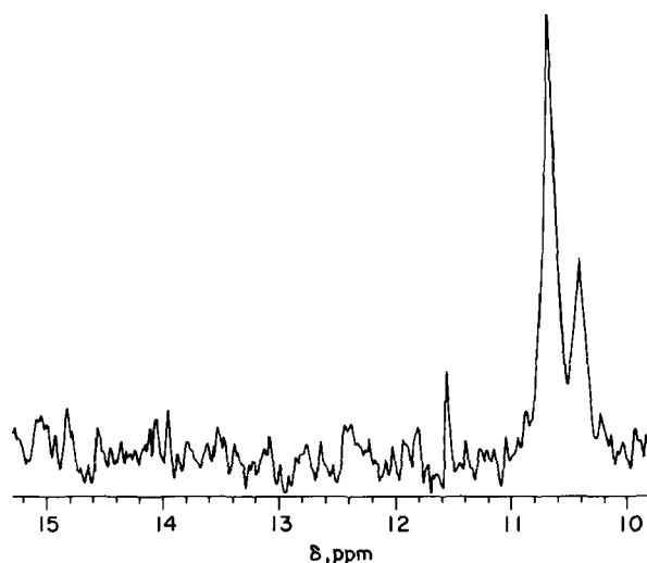
FIG. 9. A JIDS spectrum at 15^\circ\text{C} for E. coli \text{tRNA}^{\text{Phe}} . \text{tRNA}^{\text{Phe}} from E. coli grown on [1\text{-}^{15}\text{N}]\text{uracil} . The sample was dissolved in 10 mM cacodylate buffer, pH 7.0, containing 50 mM sodium chloride, 10 mM magnesium chloride, 1 mM EDTA, and 8% (v/v) deuterium oxide. A total of 1000 scans was acquired, multiplied by an exponential factor corresponding to 15 Hz of line broadening, and transformed. The absolute value spectrum is plotted.
