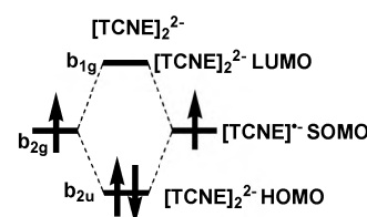
Fig. 1 MO diagram arising from the overlap of two b 2g SOMOs on each [TCNE] − forming the [TCNE] 2 2− b 2u HOMO and b 1g LUMO.
