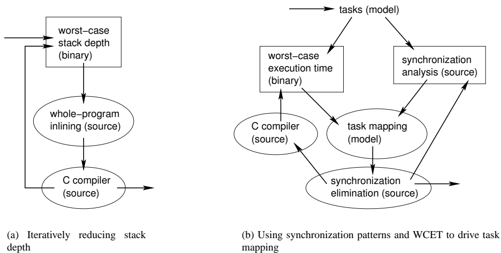
Figure 2. Two examples of vertically integrated analysis and transformation. Analyses are boxed and transformations are circled.
