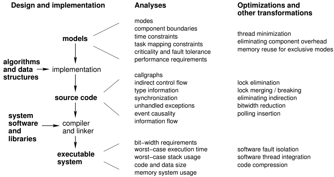
Figure 1. Program analyses and optimizations at multiple levels of abstraction
