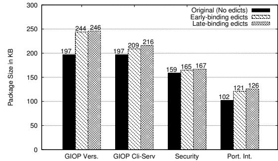
Figure 15. Per-subsystem static code sizes, before optimization
