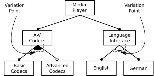
Figure 1. Hypothetical feature model for a media player
