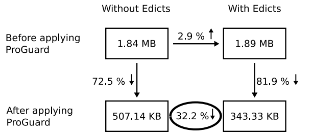
Figure 21. Early-bound edicts for application-specific JacORB
