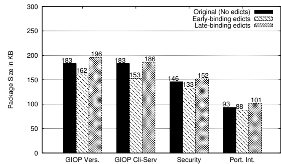
Figure 16. Per-subsystem static code sizes, after optimization
