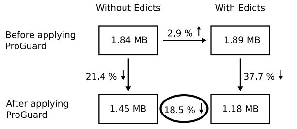
Figure 20. Early-bound edicts for API-preserving JacORB
