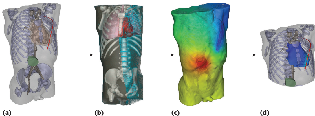
Figure 2. Pipeline for computing defibrillation potentials in children. The following are the steps required to place electrodes and compute and visualize the resulting cardiac electric potentials: (a) setting electrode configuration, (b) refinement of hexahedral mesh for electrode locations, (c) finite-element solution of electric potentials, and (d) analysis of potentials at the heart to predict defibrillation effectiveness.
