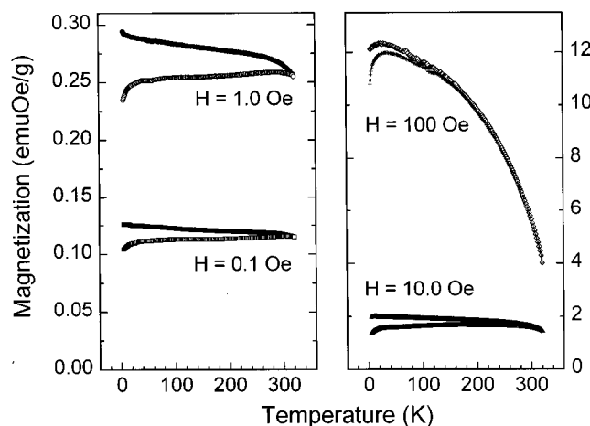
FIG. 4. Field-cooled (upper curves) and zero-field cooled (lower curves) magnetization of V[TCNE]_x film sample as function of T at different magnetic fields.
