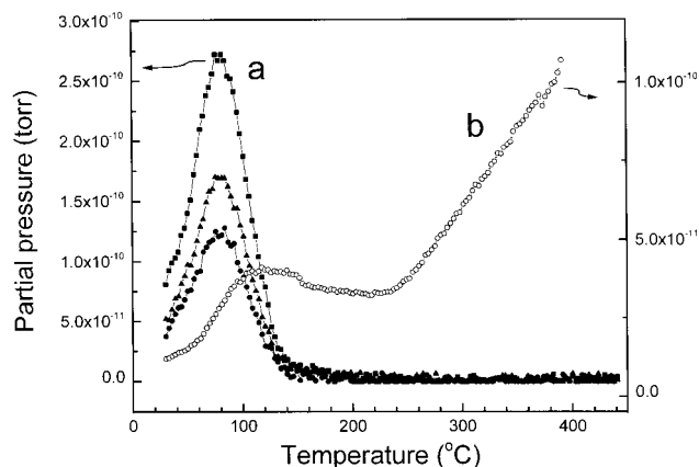
FIG. 2. Temperature dependence of the partial pressure of the ions in B : (a) originated from CH_2Cl_2 , masses = 83 ( \square ); 84 ( \triangle ); and 85 ( \bullet ) and decomposition (b) from TCNE, mass = 26 ( \circ ).
