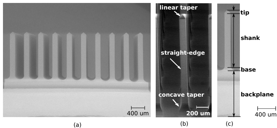
Fig. 2. SEM image of a 3D optrode array made from glass. (a) 10×10 rows of 1.5-mm long and 150- \mu\text{m} wide optrodes. (b) Profile of optrode geometry. (c) Definition of optrode sections along path of light propagation: 1-mm backplane, base extending 100 \mu\text{m} into straight-edge shank and 120- \mu\text{m} long linearly tapered tip.
