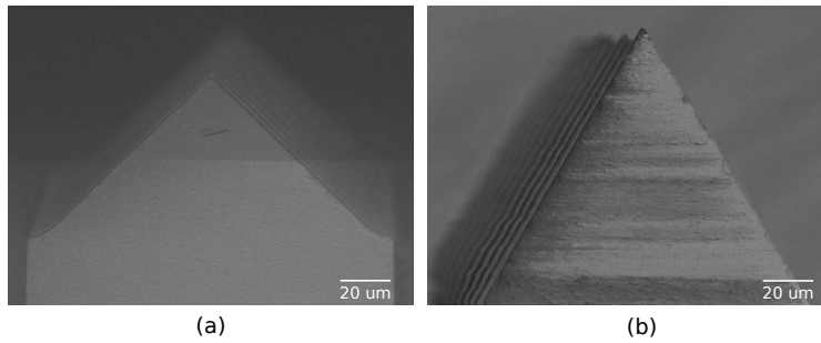
Fig. 11. Optrode tips with 45° (a) and 30° (b) taper angle with respect to the the progation direction (i.e., vertical axis). Shank width is 150 \mu\text{m} .
