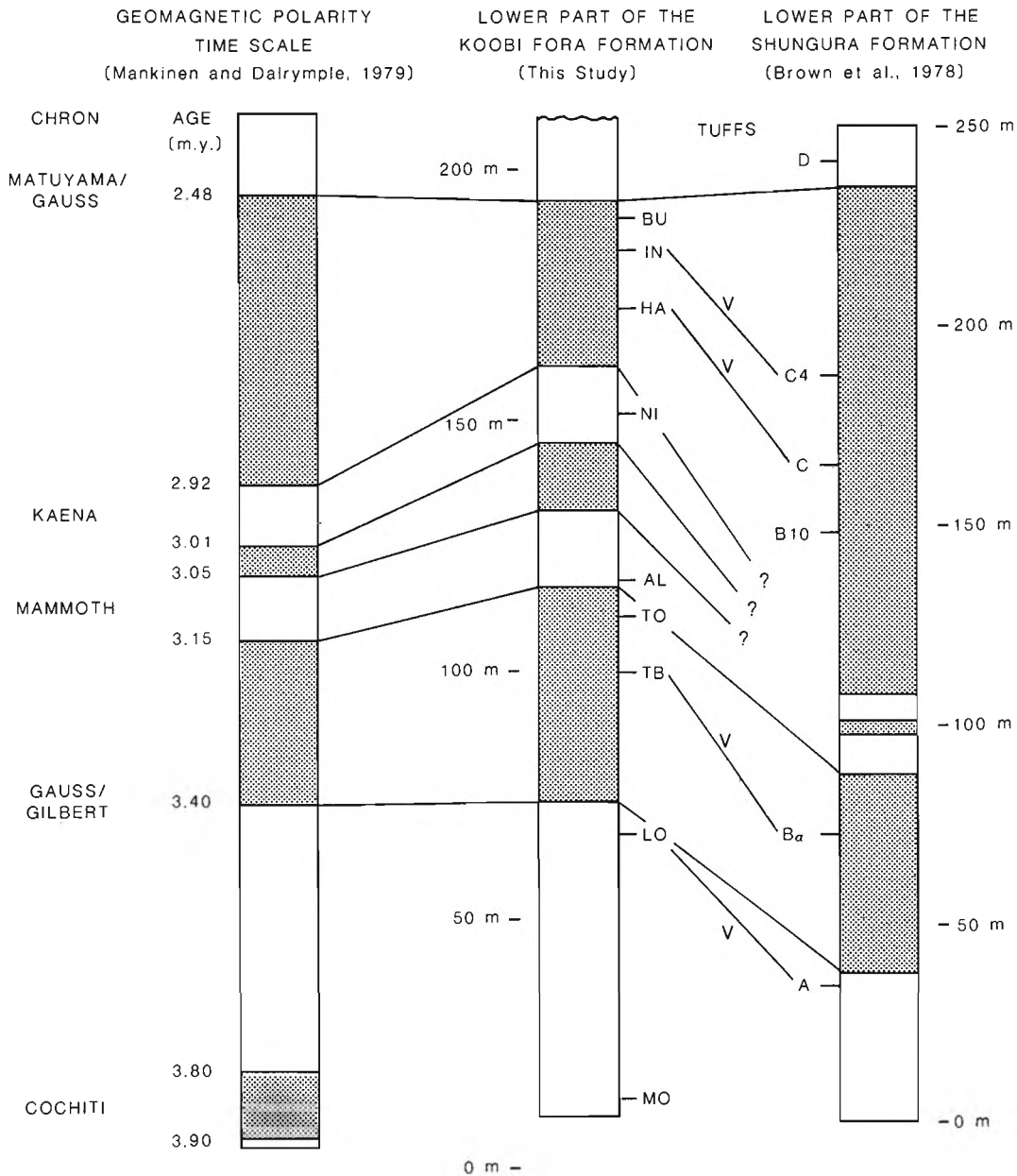
Fig. 10. Correlation of magnetozones of the lower Koobi Fora and Shungura formations with the geomagnetic polarity time scale. Stippled areas denote normal polarity. Lines with Vs denote correlative tuffs. Koobi Fora tuffs: MO, Moiti; LO, Lokochot; TB, Tulu Bor; TO, Toroto; AL, Allia; NI, Ninikaa; HA, Hasuma; IN, Ingumwai; BU, Burgi.
