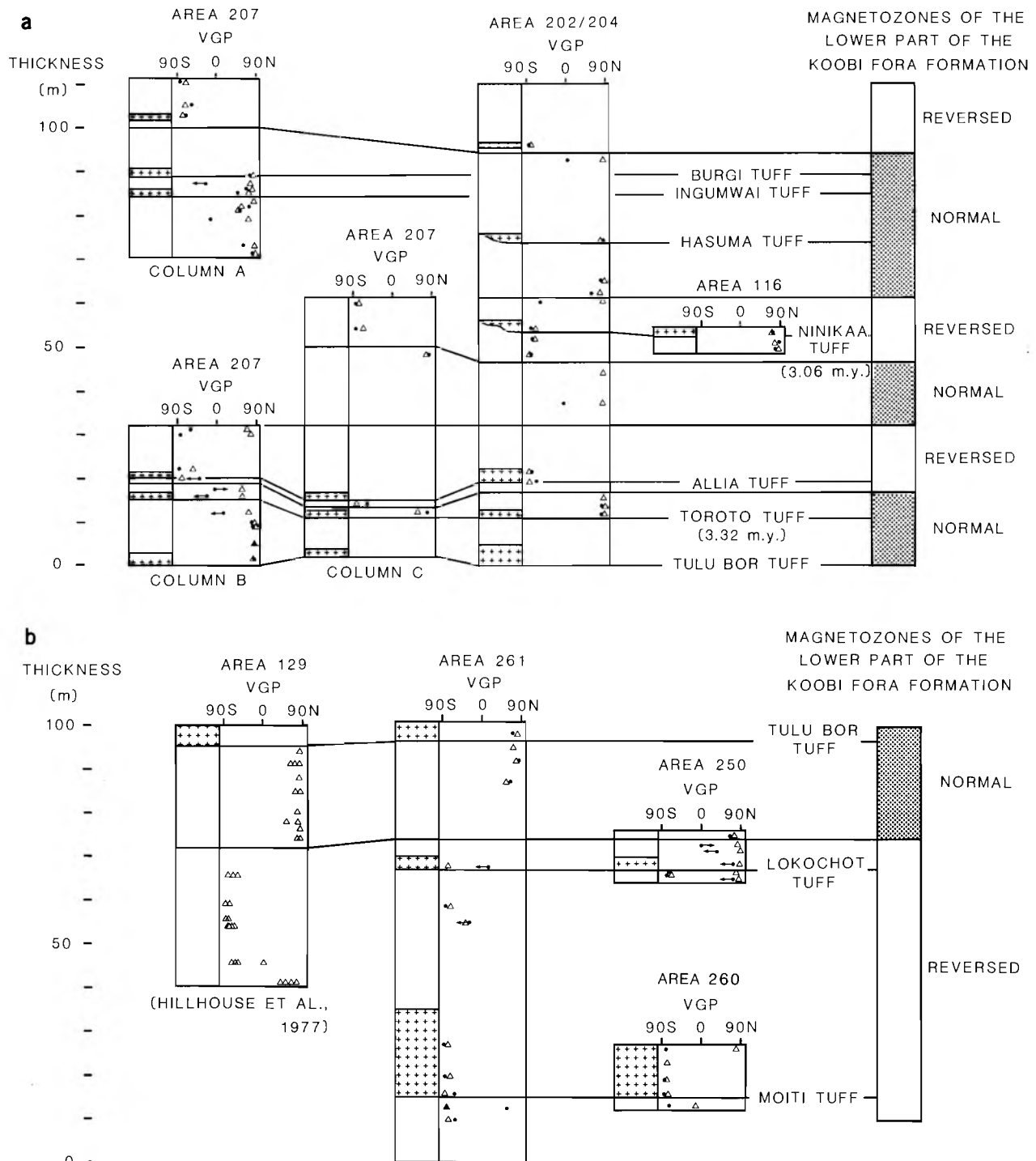
Fig. 6. Magnetostratigraphic columns of the lower part of the Koobi Fora Formation, as interpreted from the paleomagnetic columns. VGP latitudes are given for magnetic directions obtained by principal-component analysis of af (triangle) and thermal (dot) demagnetization data. Arrows indicate last sense of VGP-latitude change if direction had not stabilized. (a) Column between Tulu Bor and Burgi Tuffs. (b) Column below the Tulu Bor Tuff.
