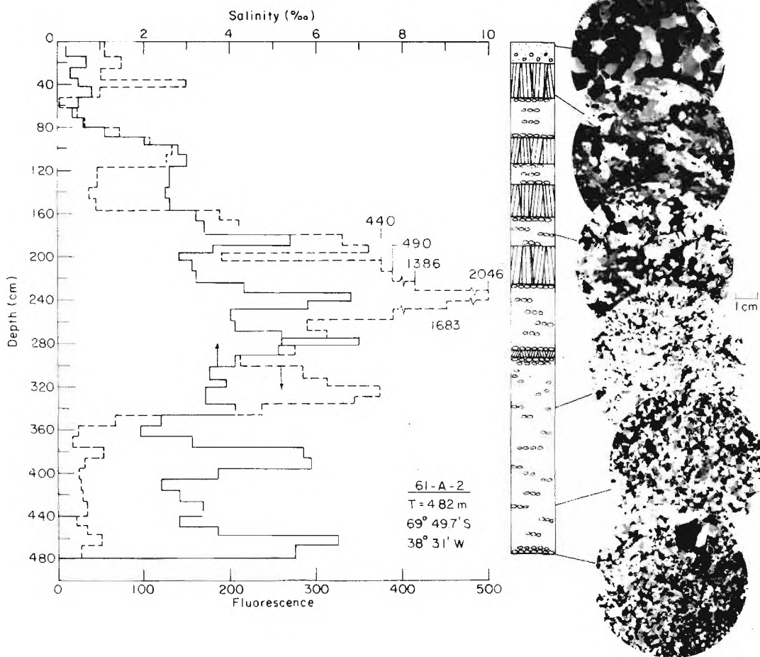
Figure 29. Salinity and fluorescence profiles, vertical structure section and horizontal thin sections of ice floe 61-A-2.
