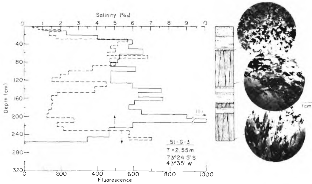
Figure 23. Salinity and fluorescence profiles, vertical structure section and horizontal thin sections of ice floe 51-G-3.
