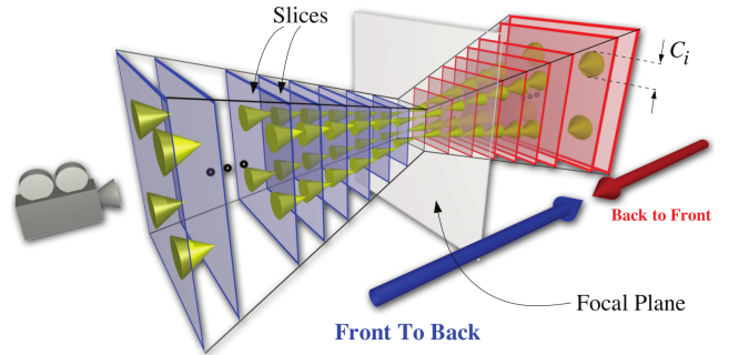
Figure 3: Geometric setup of the DVR implementation of DoF (image courtesy of Mathias Schott [26])
