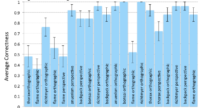
Figure 10: Average correctness for the different datasets. The datasets from left to right shows the ordering in which the videos were shown to the participants.
