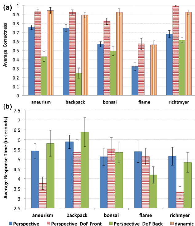
Figure 7: (a) Average correctness for the different datasets, including static and dynamic (b) Mean response time taken for the different datasets and conditions. Note: the 0 value for the flame dataset for Perspective DoF Back indicates that all answers were wrong.
