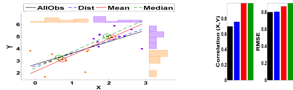
Fig. 4. Linear regression between two synthetically generated samples (orange, purple) of a bivariate distribution of random variables X and Y . Line color:: a)Black- Uses all observations (solid dots) for a linear fit. b)Blue- Proposed distribution-valued regression using marginal distributions (shown as histograms). c)Red- Using means as scalar summary statistics and d)Green- Using medians. Corresponding estimates of Correlation( X, Y ) and RMSE also shown.
