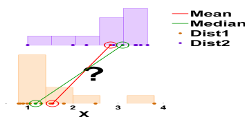
Fig. 1. Two synthetic distributions of a random variable X (dist1:orange, dist2:purple, solid dots:observed values) with the corresponding frequency histograms. Linear interpolation via classic summary statistics (mean(red) vs. median(green)) gives very different results. Data variability (depicted via circles) is discarded and hence lost at interpolated points along the fitted line.
