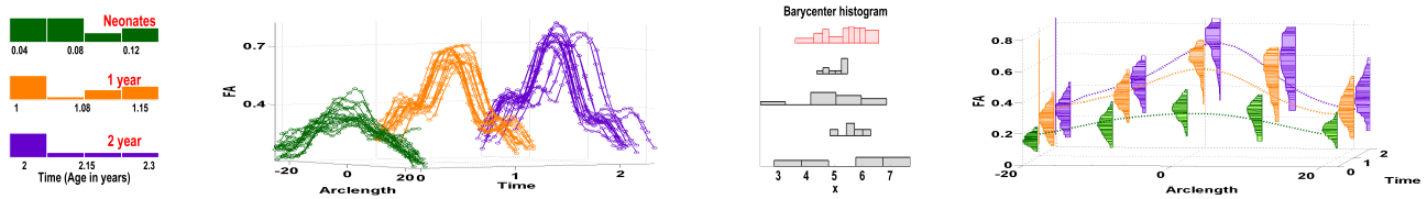
Fig. 3. Left to right: a) Distribution of ages of 15 healthy subjects within each age-group:neonate(green), 1 year(orange), 2 year(purple). b) Average FA curves from subjects within each age group with two inherent sources of variability highlighted. First, circles on each curve depict the local spatial FA distribution. Second, within each age-group, FA curves vary amongst subjects due to natural population variability. c) A barycenter histogram (topmost-red) calculated as an ‘average’ of the bottom four synthetic histograms. d) At each arc length location along the tract, FA histograms of all subjects within an age-group are averaged to create a barycenter histogram (only a few locations shown).
