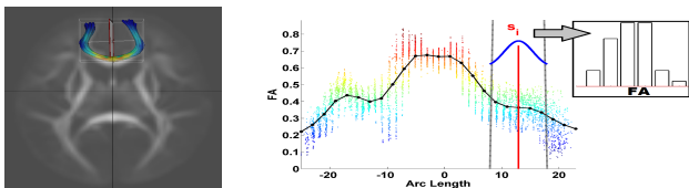
Fig. 2. Left: 3D visualization of the genu white matter tract from a single DTI scan. Right: Diffusion values (FA) assembled along genu tract's length (scatter points colored by FA) with the corresponding cross-sectional average FA curve (black) [6]. Kernel weights are applied to compute a histogram of the spatial FA distribution within a kernel window centered at arc-length location s_i along the tract.
