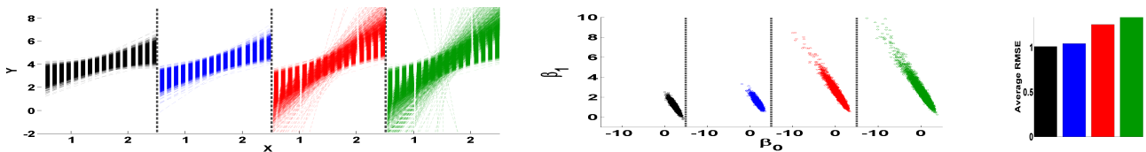
Fig. 5. 10,000 repetitions of synthetic regression experiment (Fig.4). Regression results: All Observations (black), Distribution-valued (blue), mean (red), median (green). Left to right: a) Linear fits obtained from 10,000 repetitions. b) Estimated regression coefficients \beta_1 :slope, \beta_0 :intercept (extreme outlier coefficients from mean/median regression omitted in the plot). c) Average of 10,000 RMSE estimates.
