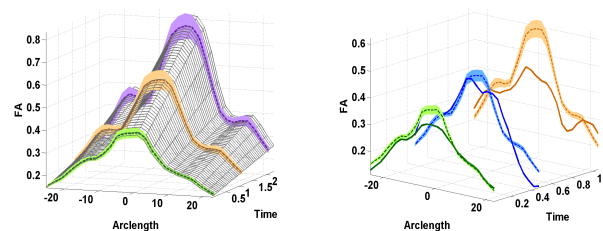
Fig. 6. Left: Continuous spatiotemporal normative FA evolution (genu tract). Estimated mean FA: gray, standard deviation bounds: neonate (green), 1 year (orange), 2 year (purple). Right: Krabbe’s subject’s average FA curves (solid lines) at 14 days, 6 month (blue), 1 year. Corresponding population mean (dashed line) and standard deviation shown for matched age-groups (blue: 6 month \pm 2 weeks).
